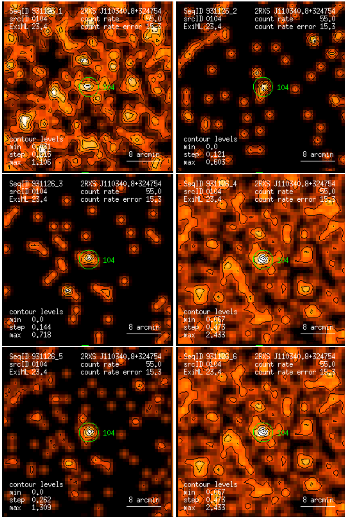
Figure 104: RASS 931126: detection 0104: band rate images, Gaussian filter: (1) PSPC channels 11 – 41, (2) 52 – 90, (3) 91 – 201, (4) 11 – 235, (5) 52 – 201, (6) 11 – 201. Broad band rates in counts/ks. Band rate contour levels in counts/ks/arcmin 2 .
