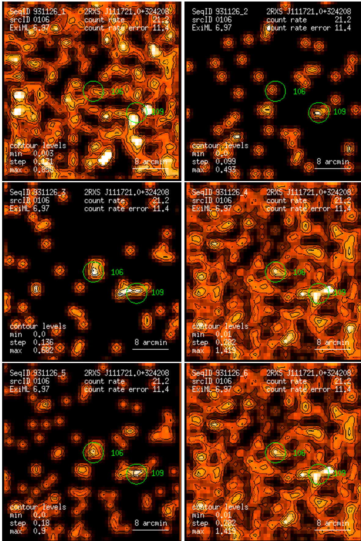
Figure 106: RASS 931126: detection 0106: band rate images, Gaussian filter: (1) PSPC channels 11 – 41, (2) 52 – 90, (3) 91 – 201, (4) 11 – 235, (5) 52 – 201, (6) 11 – 201. Broad band rates in counts/ks. Band rate contour levels in counts/ks/arcmin 2 .
