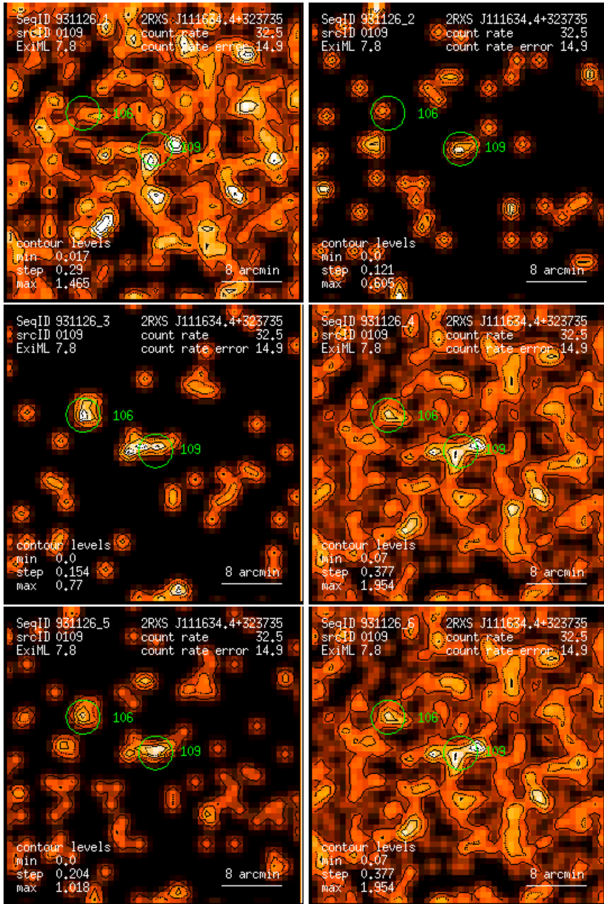
Figure 109: RASS 931126: detection 0109: band rate images, Gaussian filter: (1) PSPC channels 11 – 41, (2) 52 – 90, (3) 91 – 201, (4) 11 – 235, (5) 52 – 201, (6) 11 – 201. Broad band rates in counts/ks. Band rate contour levels in counts/ks/arcmin 2 .
