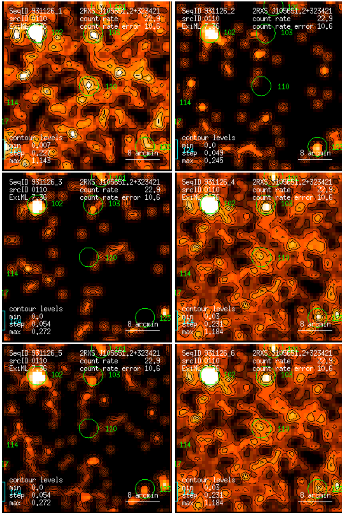
Figure 110: RASS 931126: detection 0110: band rate images, Gaussian filter: (1) PSPC channels 11 – 41, (2) 52 – 90, (3) 91 – 201, (4) 11 – 235, (5) 52 – 201, (6) 11 – 201. Broad band rates in counts/ks. Band rate contour levels in counts/ks/arcmin 2 .
