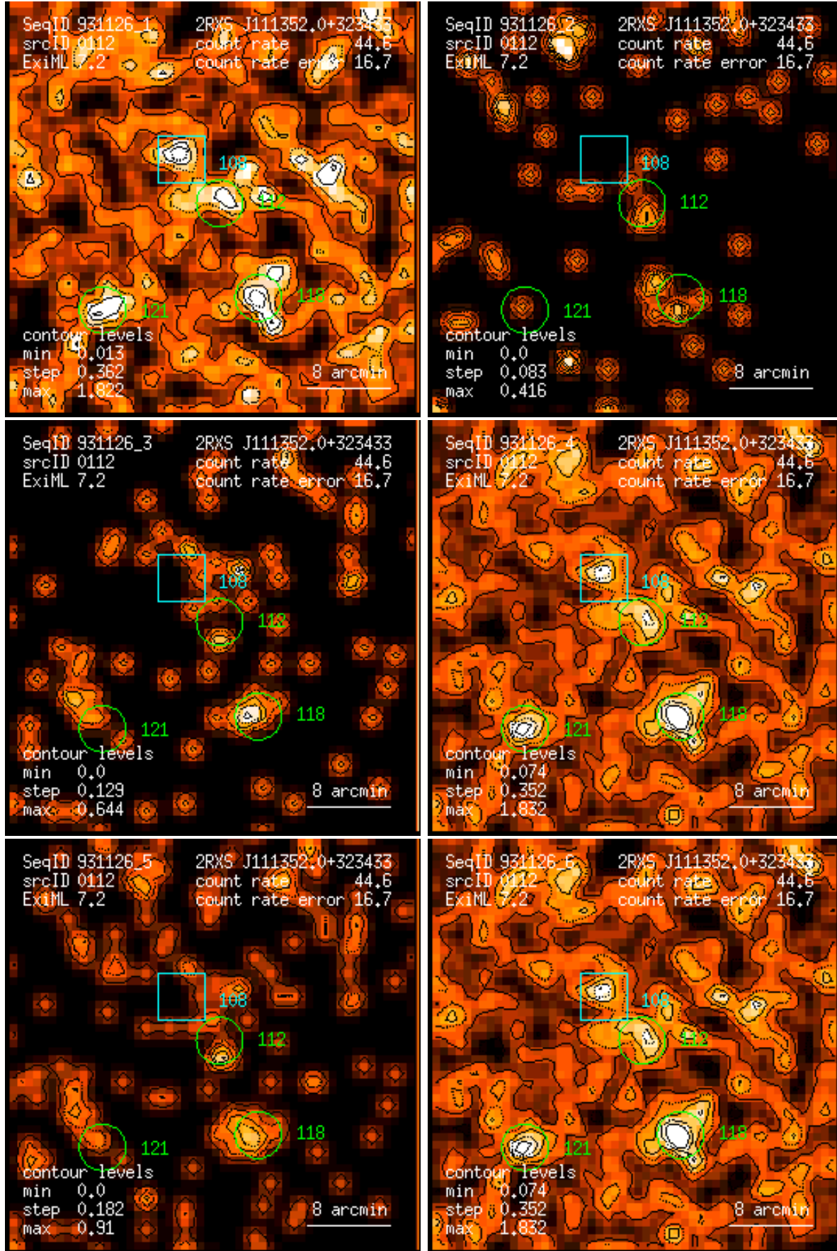
Figure 112: RASS 931126: detection 0112: band rate images, Gaussian filter: (1) PSPC channels 11 – 41, (2) 52 – 90, (3) 91 – 201, (4) 11 – 235, (5) 52 – 201, (6) 11 – 201. Broad band rates in counts/ks. Band rate contour levels in counts/ks/arcmin 2 .
