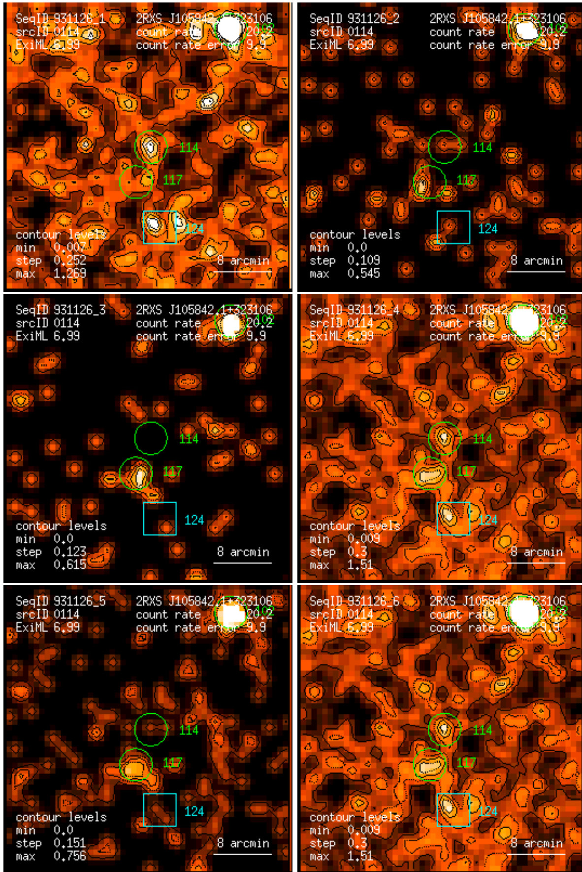
Figure 114: RASS 931126: detection 0114: band rate images, Gaussian filter: (1) PSPC channels 11 – 41, (2) 52 – 90, (3) 91 – 201, (4) 11 – 235, (5) 52 – 201, (6) 11 – 201. Broad band rates in counts/ks. Band rate contour levels in counts/ks/arcmin 2 .
