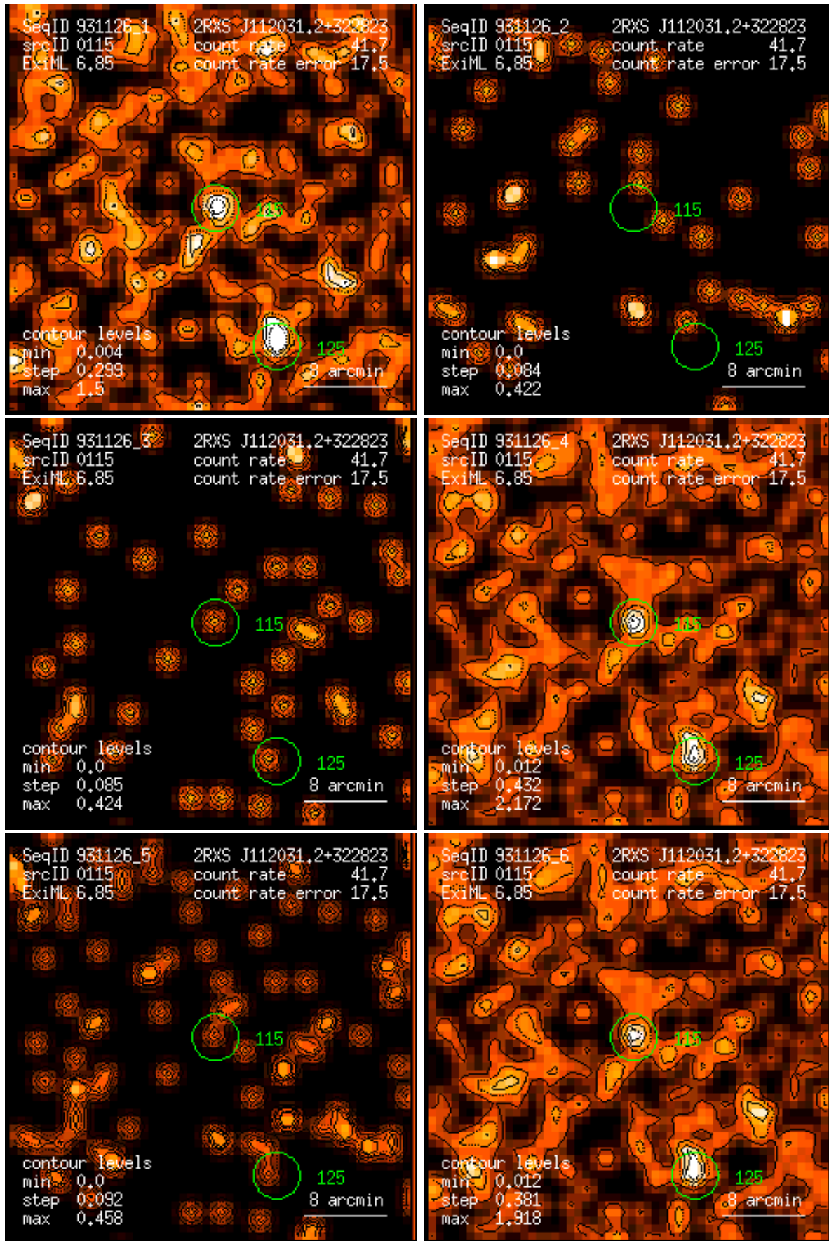
Figure 115: RASS 931126: detection 0115: band rate images, Gaussian filter: (1) PSPC channels 11 – 41, (2) 52 – 90, (3) 91 – 201, (4) 11 – 235, (5) 52 – 201, (6) 11 – 201. Broad band rates in counts/ks. Band rate contour levels in counts/ks/arcmin 2 .
