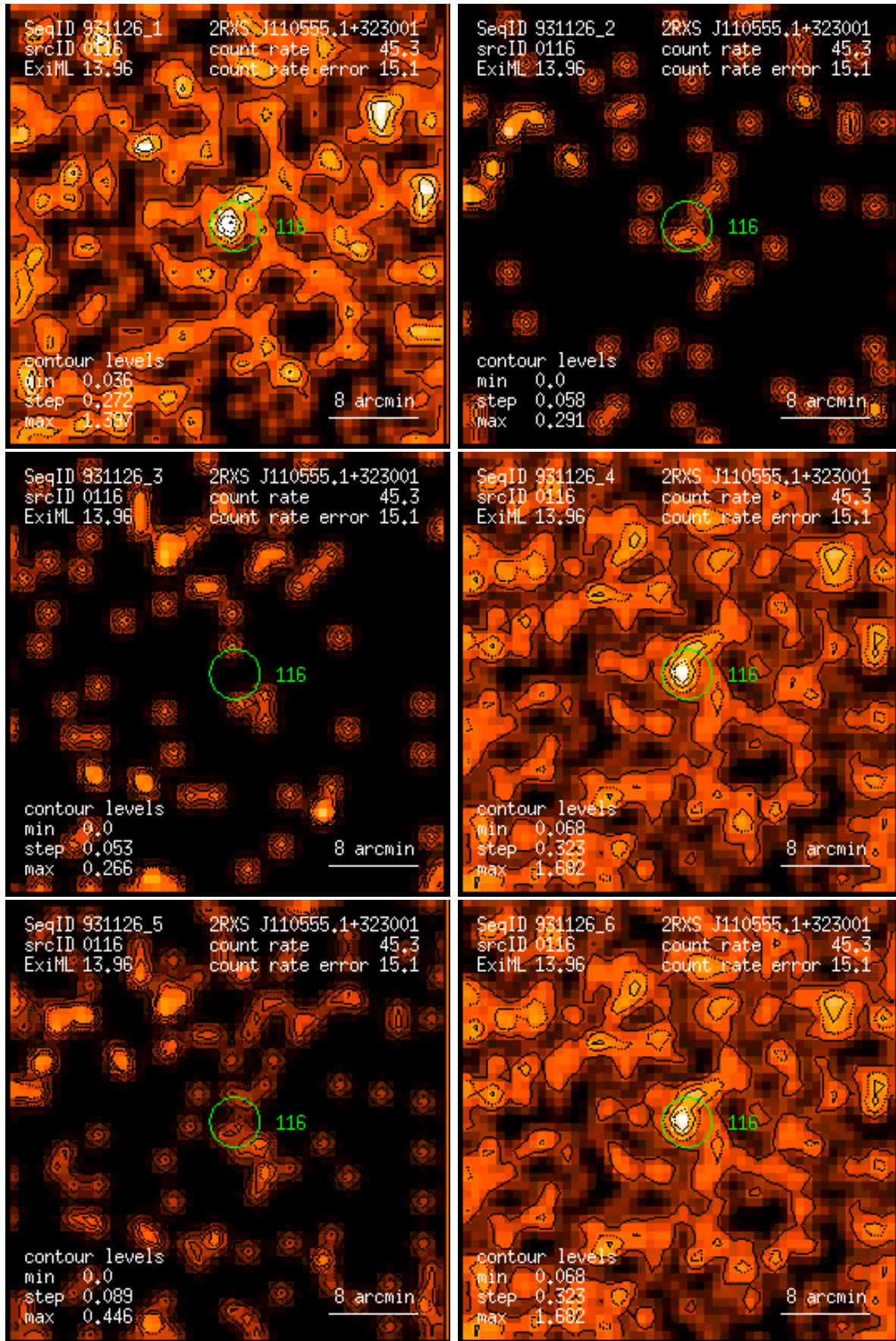
Figure 116: RASS 931126: detection 0116: band rate images, Gaussian filter: (1) PSPC channels 11 – 41, (2) 52 – 90, (3) 91 – 201, (4) 11 – 235, (5) 52 – 201, (6) 11 – 201. Broad band rates in counts/ks. Band rate contour levels in counts/ks/arcmin 2 .
