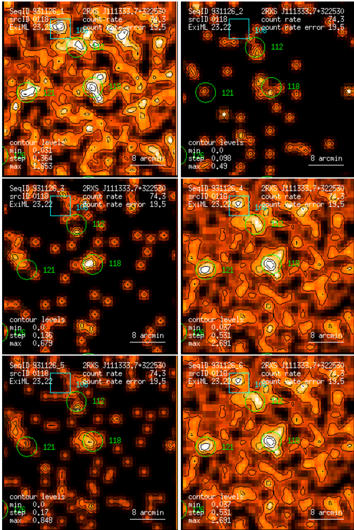
Figure 118: RASS 931126: detection 0118: band rate images, Gaussian filter: (1) PSPC channels 11 – 41, (2) 52 – 90, (3) 91 – 201, (4) 11 – 235, (5) 52 – 201, (6) 11 – 201. Broad band rates in counts/ks. Band rate contour levels in counts/ks/arcmin 2 .
