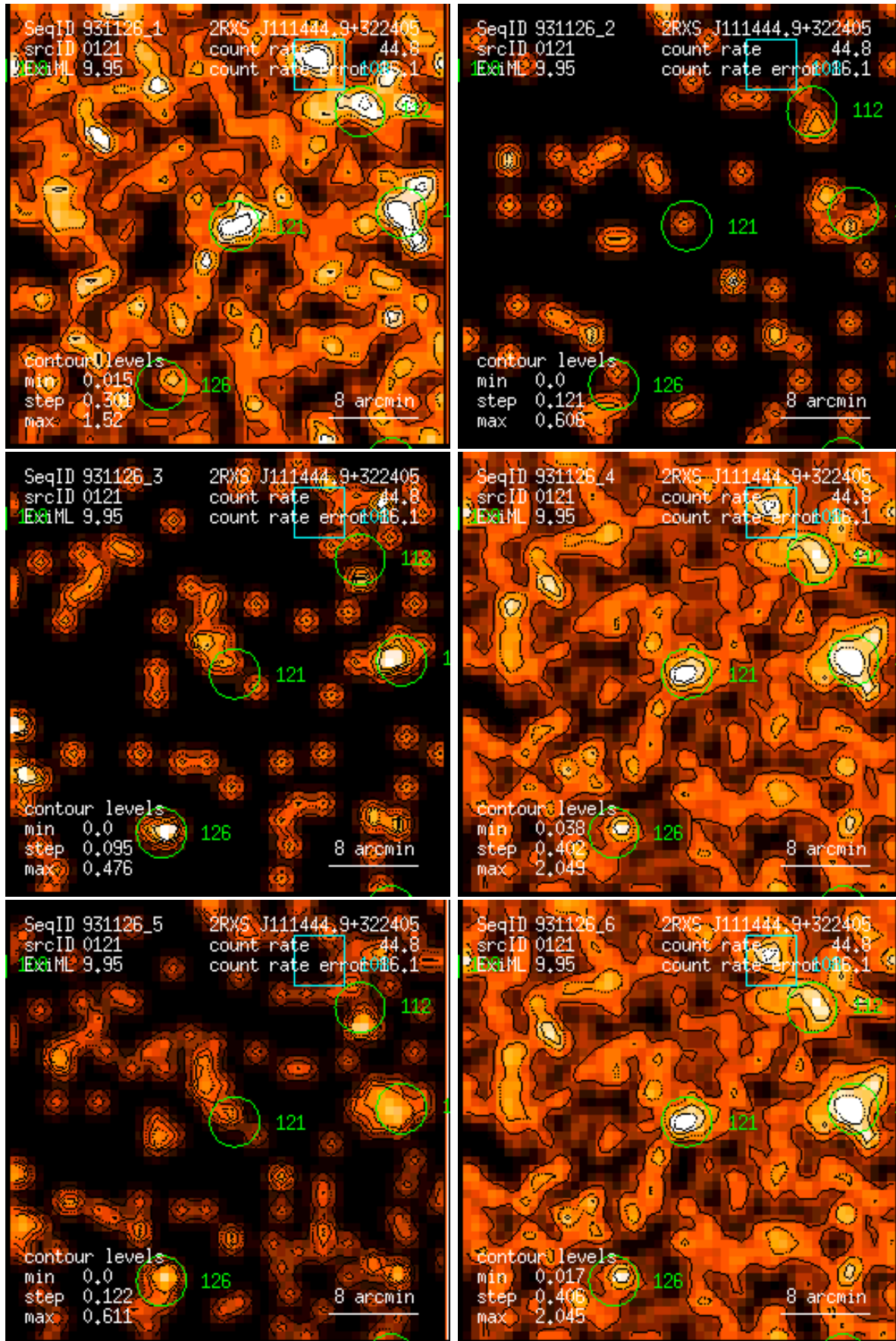
Figure 121: RASS 931126: detection 0121: band rate images, Gaussian filter: (1) PSPPC channels 11 – 41, (2) 52 – 90, (3) 91 – 201, (4) 11 – 235, (5) 52 – 201, (6) 11 – 201. Broad band rates in counts/ks. Band rate contour levels in counts/ks/arcmin 2 .
