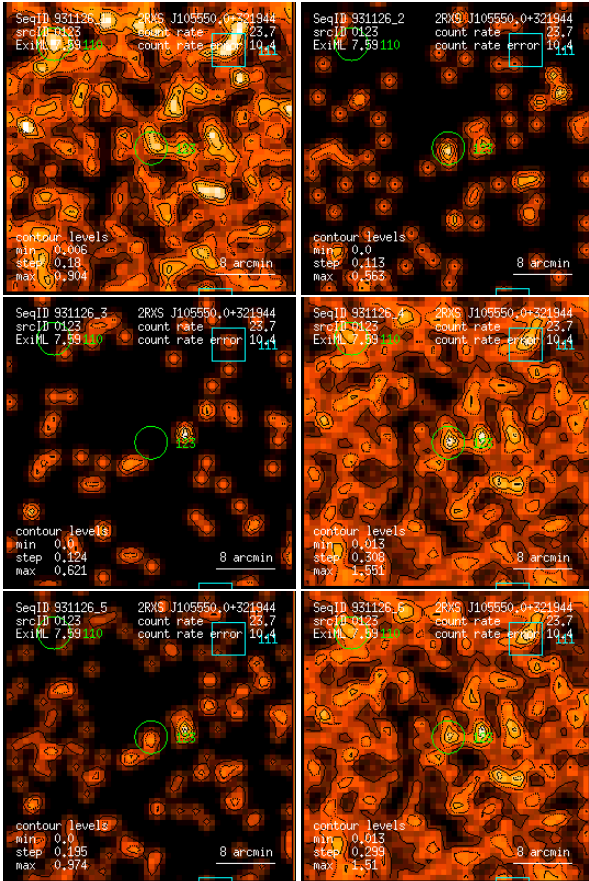
Figure 123: RASS 931126: detection 0123: band rate images, Gaussian filter: (1) PSPC channels 11 – 41, (2) 52 – 90, (3) 91 – 201, (4) 11 – 235, (5) 52 – 201, (6) 11 – 201. Broad band rates in counts/ks. Band rate contour levels in counts/ks/arcmin 2 .
