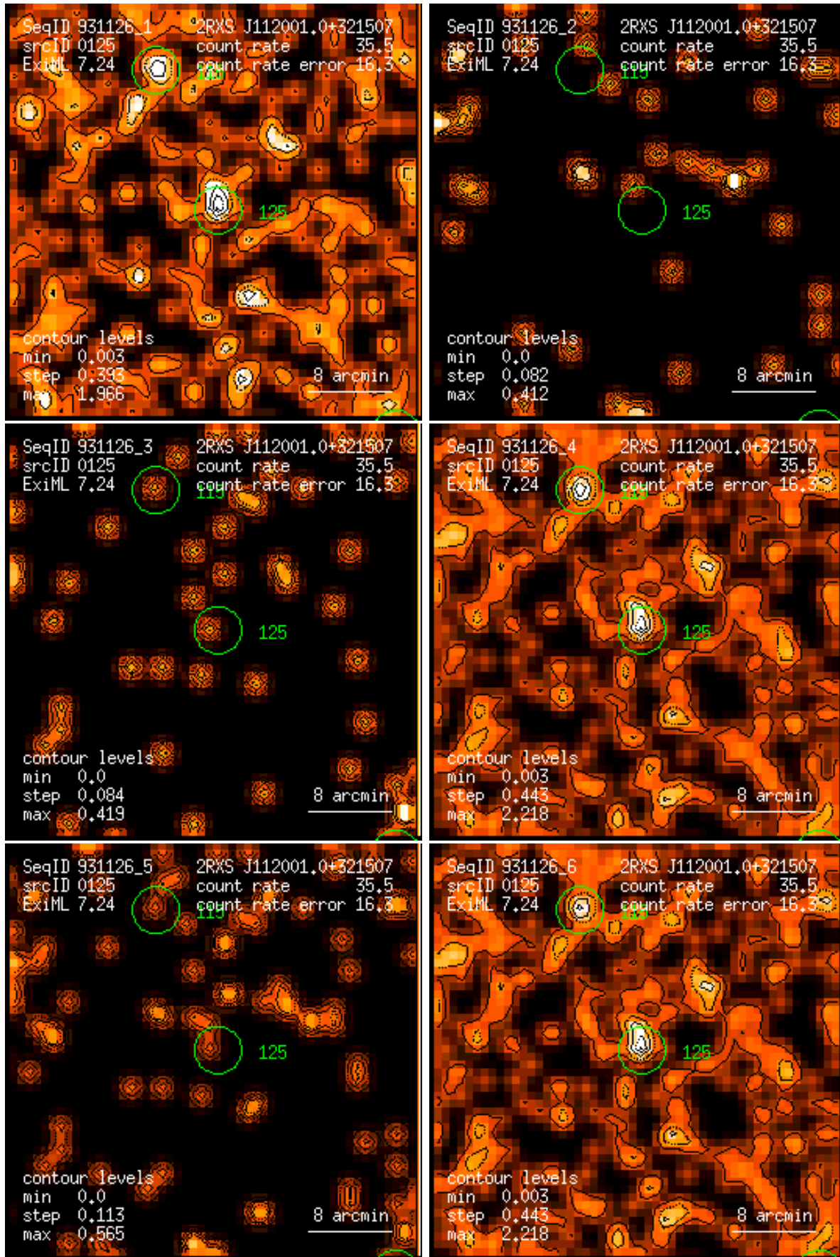
Figure 125: RASS 931126: detection 0125: band rate images, Gaussian filter: (1) PSPC channels 11 – 41, (2) 52 – 90, (3) 91 – 201, (4) 11 – 235, (5) 52 – 201, (6) 11 – 201. Broad band rates in counts/ks. Band rate contour levels in counts/ks/arcmin 2 .
