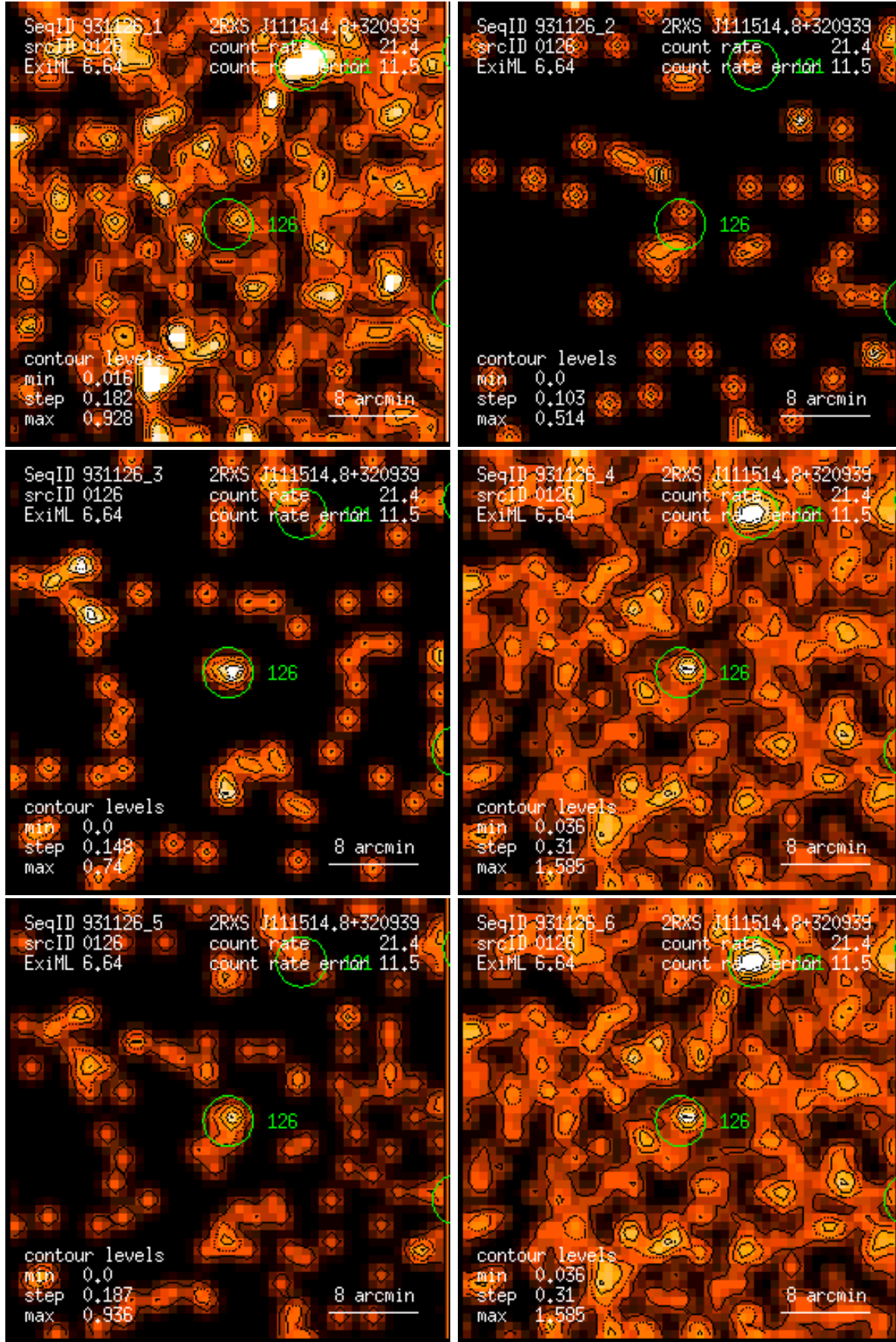
Figure 126: RASS 931126: detection 0126: band rate images, Gaussian filter: (1) PSPC channels 11 – 41, (2) 52 – 90, (3) 91 – 201, (4) 11 – 235, (5) 52 – 201, (6) 11 – 201. Broad band rates in counts/ks. Band rate contour levels in counts/ks/arcmin 2 .
