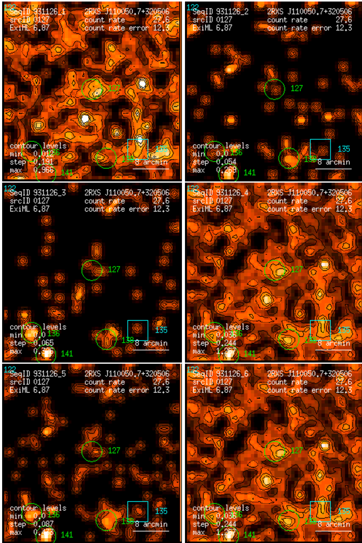
Figure 127: RASS 931126: detection 0127: band rate images, Gaussian filter: (1) PSPC channels 11 – 41, (2) 52 – 90, (3) 91 – 201, (4) 11 – 235, (5) 52 – 201, (6) 11 – 201. Broad band rates in counts/ks. Band rate contour levels in counts/ks/arcmin 2 .
