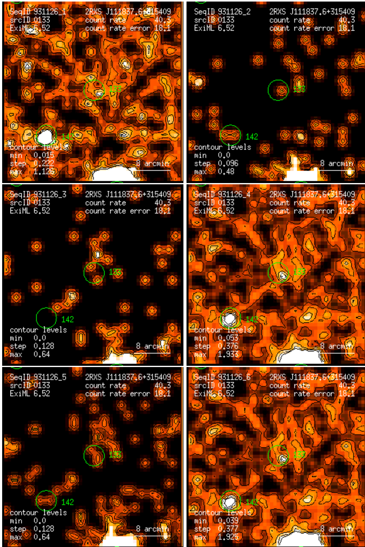
Figure 133: RASS 931126: detection 0133: band rate images, Gaussian filter: (1) PSPC channels 11 – 41, (2) 52 – 90, (3) 91 – 201, (4) 11 – 235, (5) 52 – 201, (6) 11 – 201. Broad band rates in counts/ks. Band rate contour levels in counts/ks/arcmin 2 .
