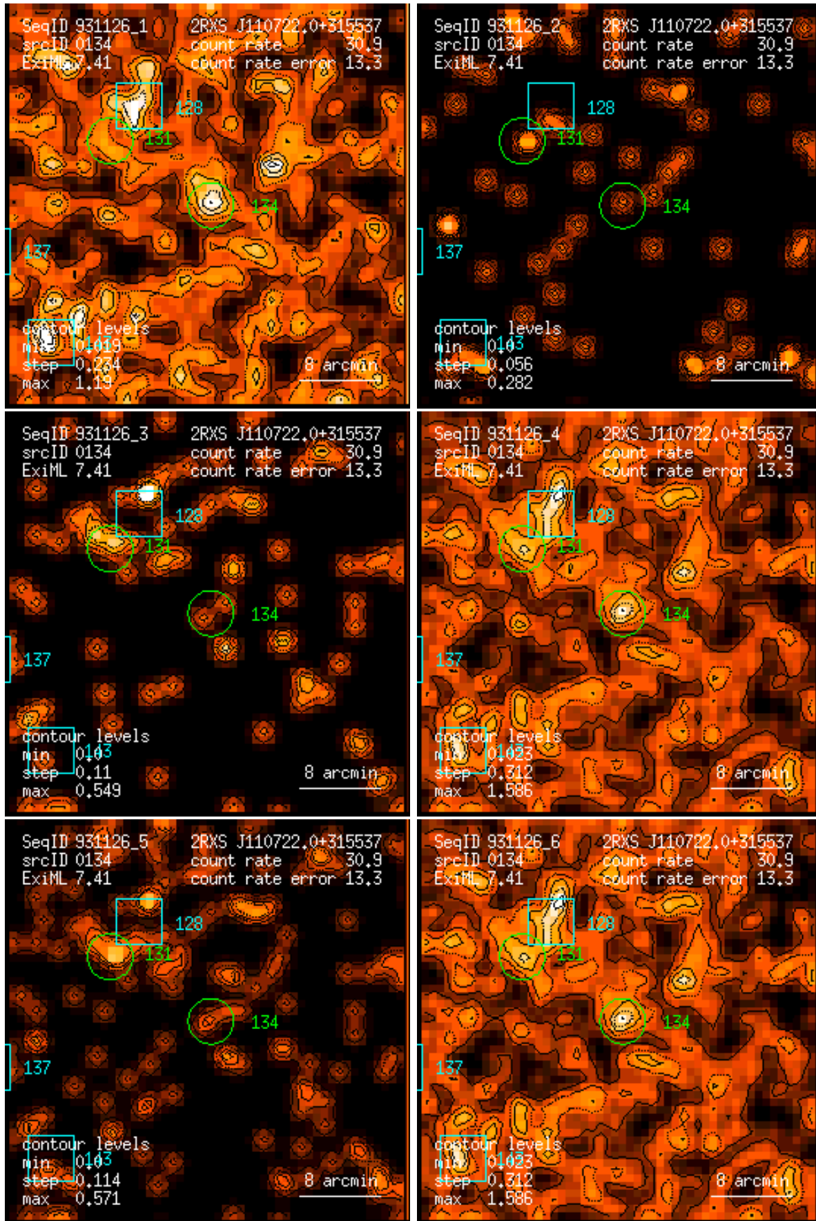
Figure 134: RASS 931126: detection 0134: band rate images, Gaussian filter: (1) PSPC channels 11 – 41, (2) 52 – 90, (3) 91 – 201, (4) 11 – 235, (5) 52 – 201, (6) 11 – 201. Broad band rates in counts/ks. Band rate contour levels in counts/ks/arcmin 2 .
