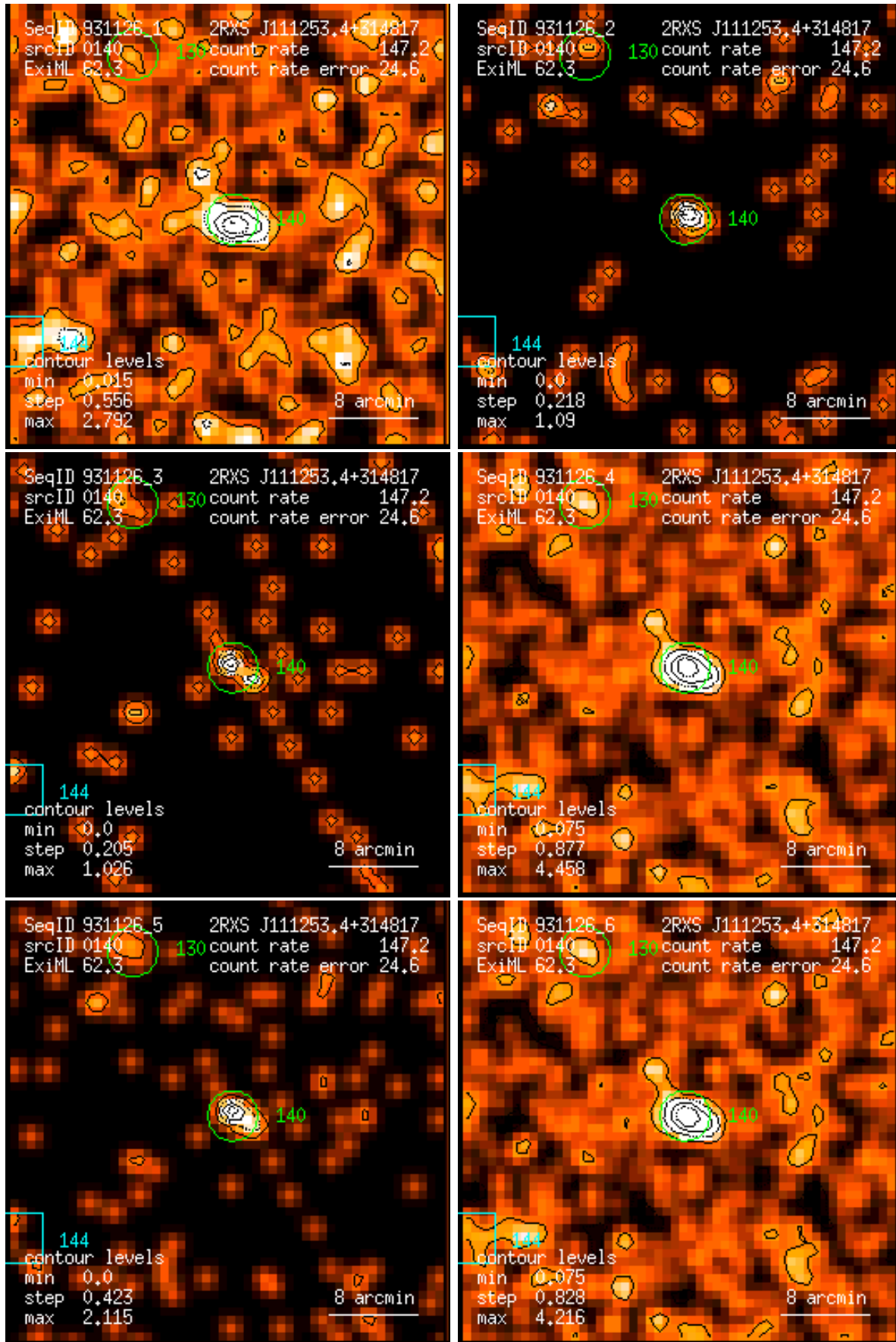
Figure 140: RASS 931126: detection 0140: band rate images, Gaussian filter: (1) PSPC channels 11 – 41, (2) 52 – 90, (3) 91 – 201, (4) 11 – 235, (5) 52 – 201, (6) 11 – 201. Broad band rates in counts/ks. Band rate contour levels in counts/ks/arcmin 2 .
