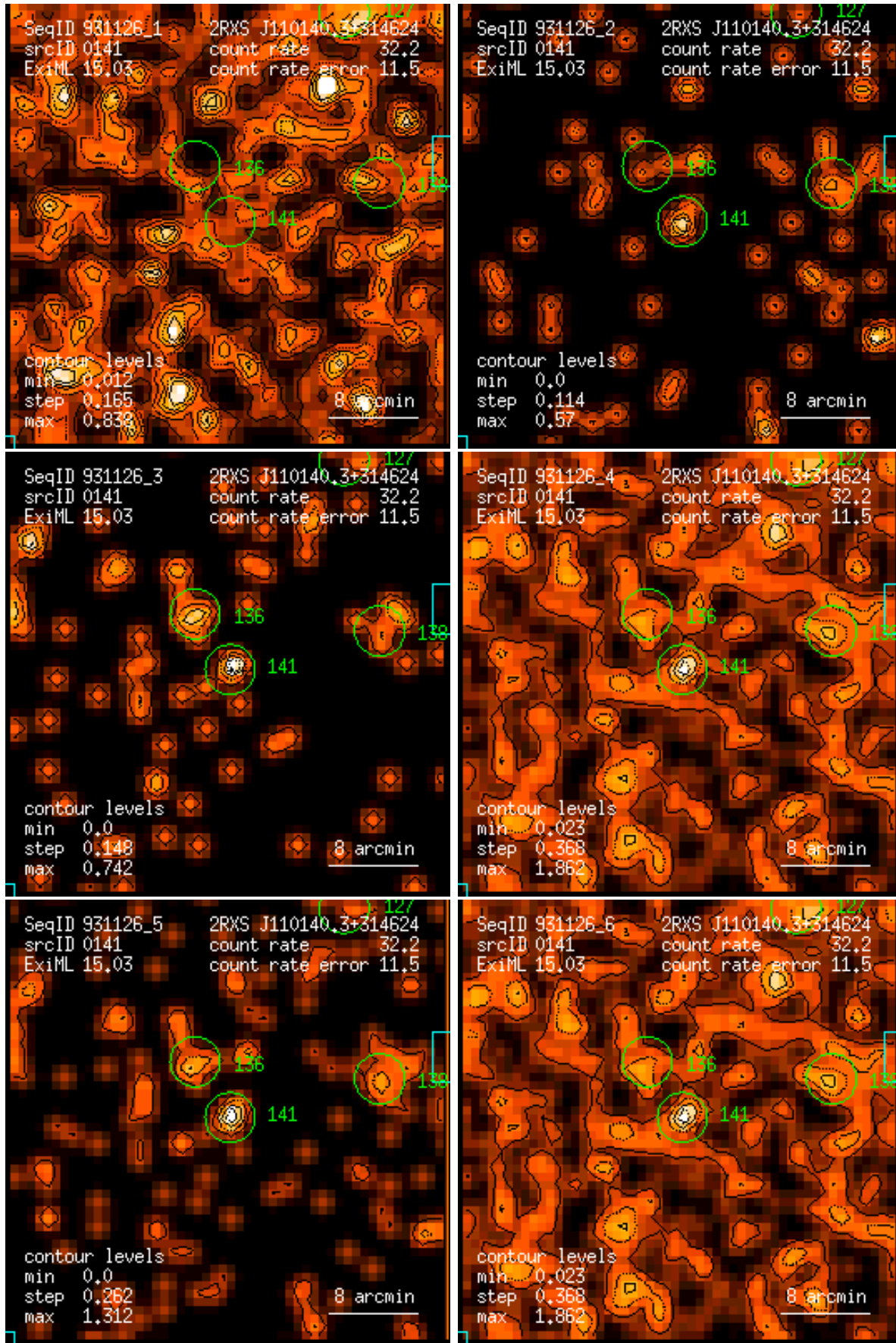
Figure 141: RASS 931126: detection 0141: band rate images, Gaussian filter: (1) PSPC channels 11 – 41, (2) 52 – 90, (3) 91 – 201, (4) 11 – 235, (5) 52 – 201, (6) 11 – 201. Broad band rates in counts/ks. Band rate contour levels in counts/ks/arcmin 2 .
