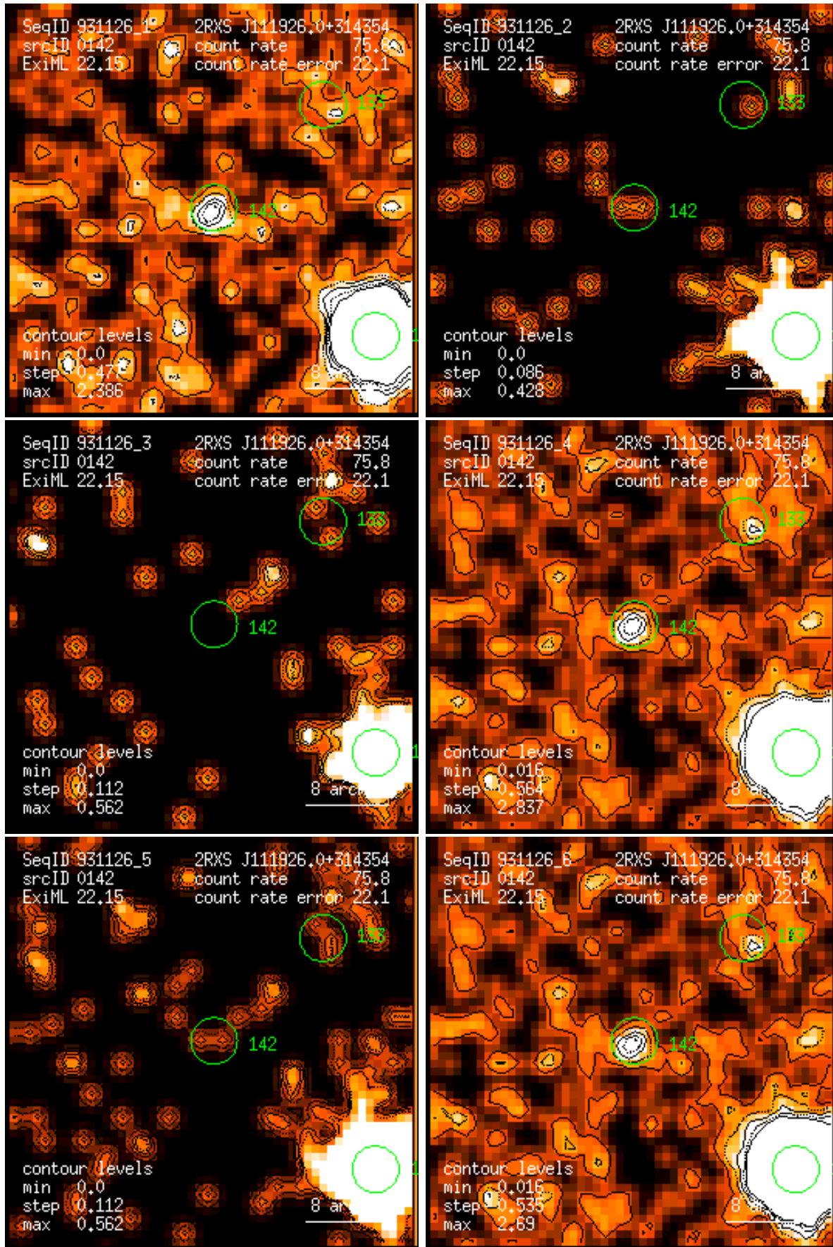
Figure 142: RASS 931126: detection 0142: band rate images, Gaussian filter: (1) PSPC channels 11 – 41, (2) 52 – 90, (3) 91 – 201, (4) 11 – 235, (5) 52 – 201, (6) 11 – 201. Broad band rates in counts/ks. Band rate contour levels in counts/ks/arcmin 2 .
