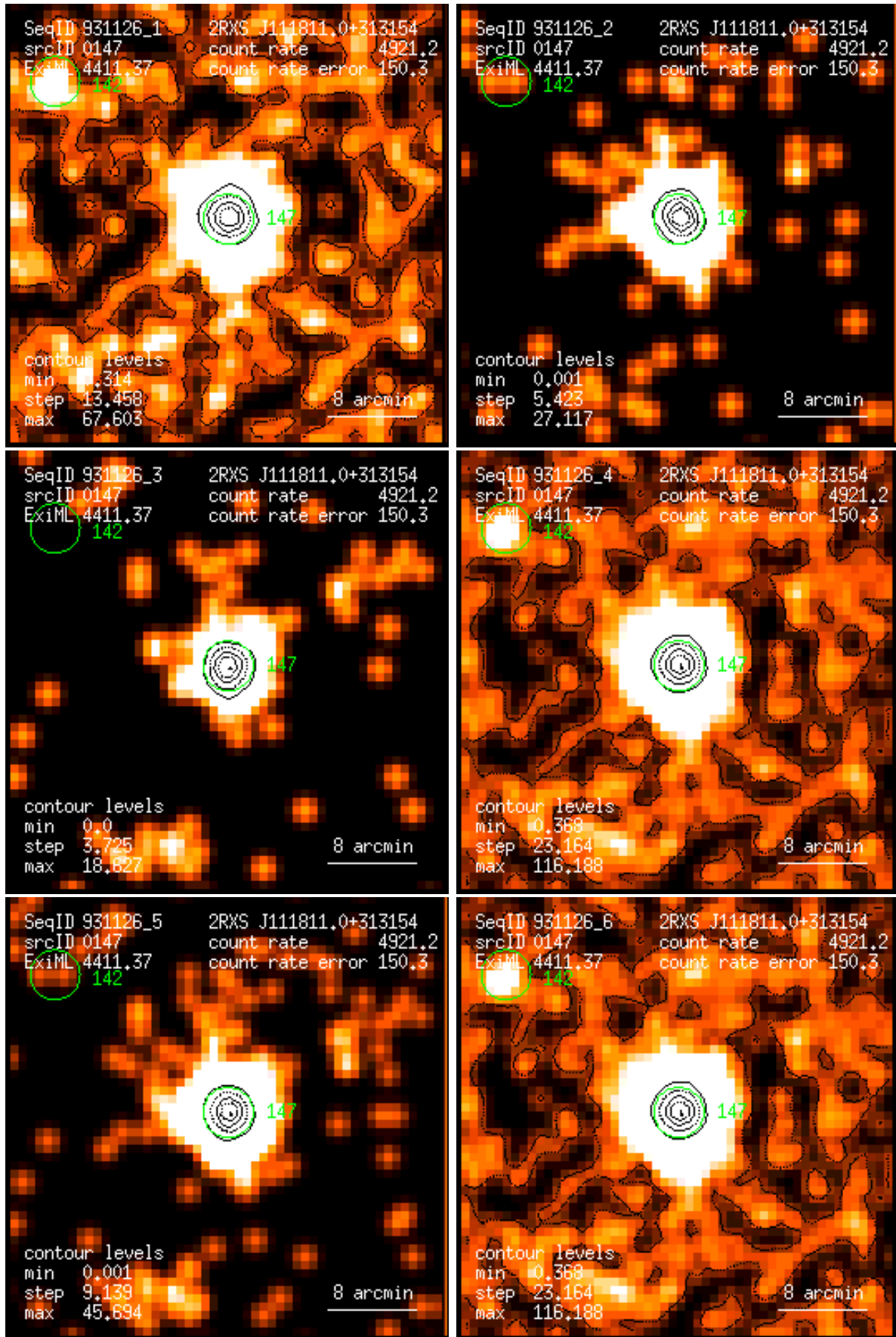
Figure 147: RASS 931126: detection 0147: band rate images, Gaussian filter: (1) PSPC channels 11 – 41, (2) 52 – 90, (3) 91 – 201, (4) 11 – 235, (5) 52 – 201, (6) 11 – 201. Broad band rates in counts/ks. Band rate contour levels in counts/ks/arcmin 2 .
