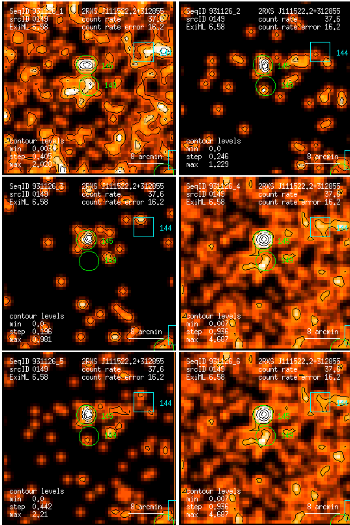
Figure 149: RASS 931126: detection 0149: band rate images, Gaussian filter: (1) PSPC channels 11 – 41, (2) 52 – 90, (3) 91 – 201, (4) 11 – 235, (5) 52 – 201, (6) 11 – 201. Broad band rates in counts/ks. Band rate contour levels in counts/ks/arcmin 2 .
