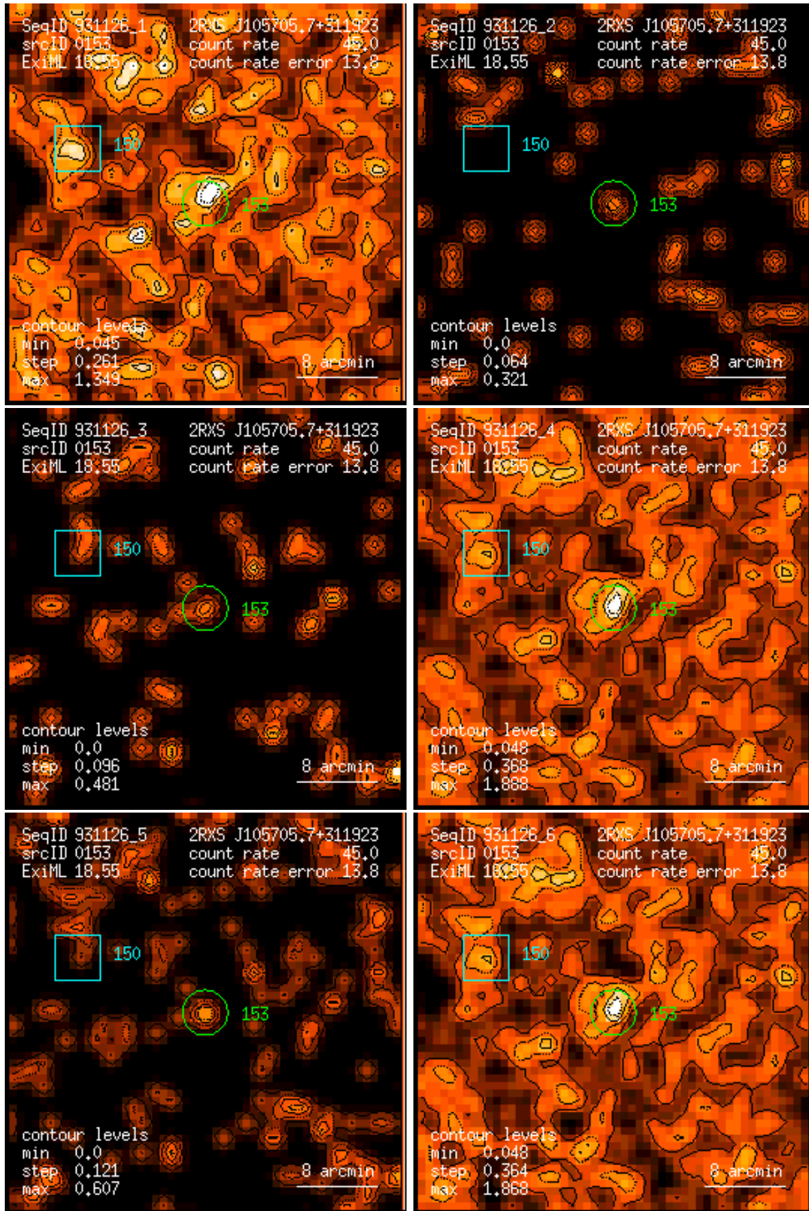
Figure 153: RASS 931126: detection 0153: band rate images, Gaussian filter: (1) PSPC channels 11 – 41, (2) 52 – 90, (3) 91 – 201, (4) 11 – 235, (5) 52 – 201, (6) 11 – 201. Broad band rates in counts/ks. Band rate contour levels in counts/ks/arcmin 2 .
