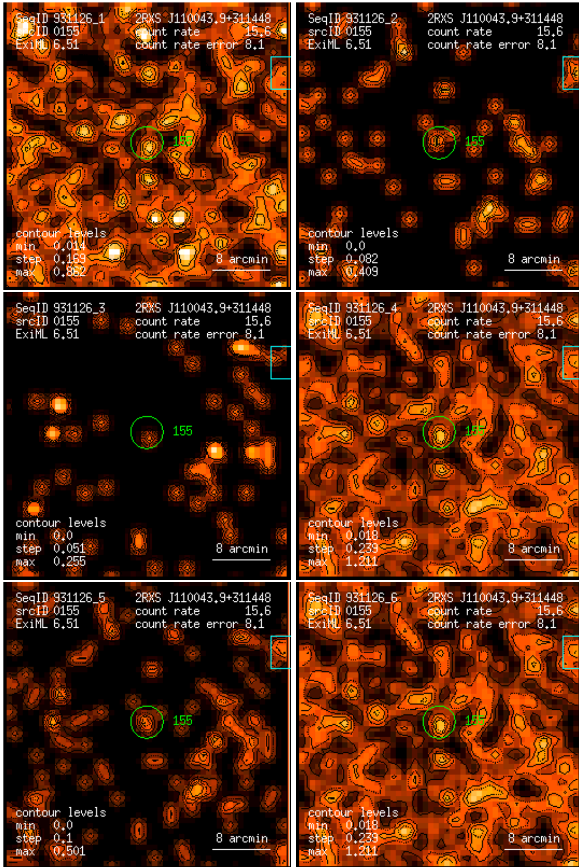
Figure 155: RASS 931126: detection 0155: band rate images, Gaussian filter: (1) PSPC channels 11 – 41, (2) 52 – 90, (3) 91 – 201, (4) 11 – 235, (5) 52 – 201, (6) 11 – 201. Broad band rates in counts/ks. Band rate contour levels in counts/ks/arcmin 2 .
