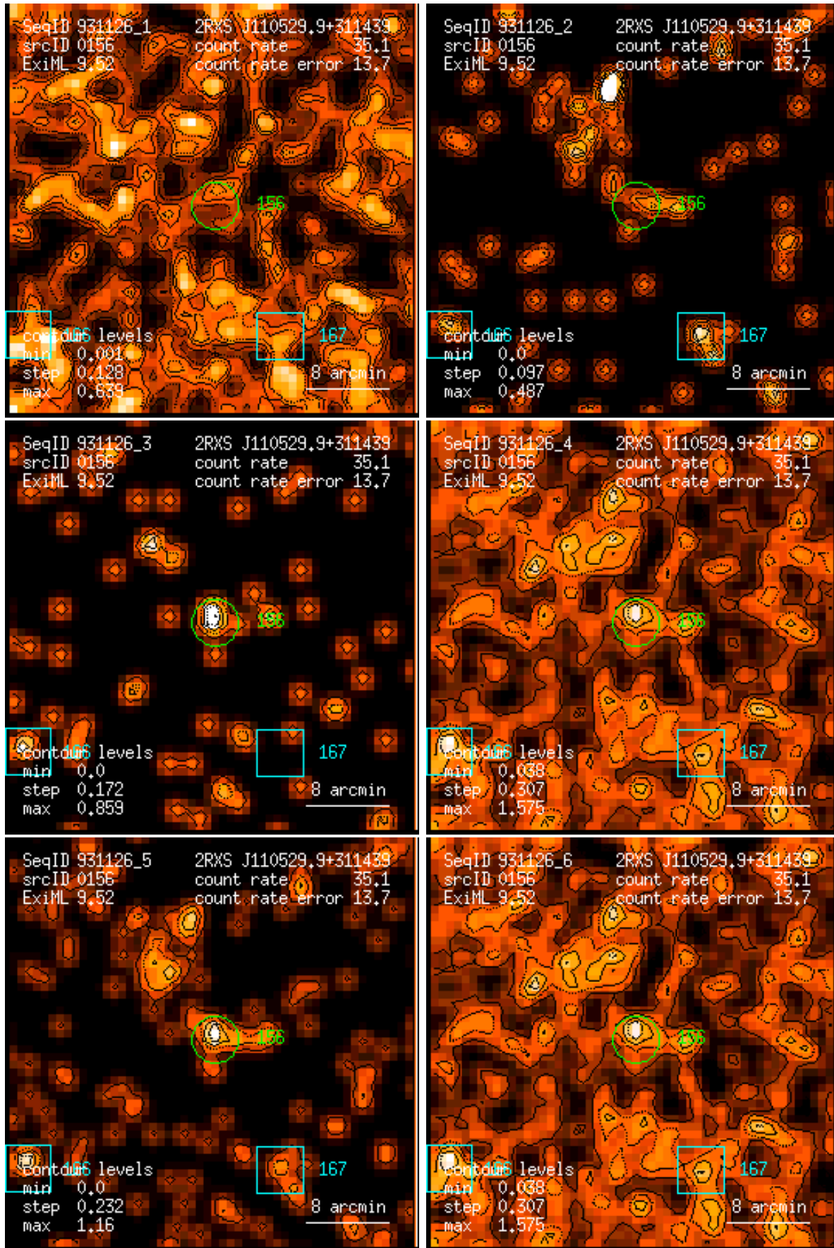
Figure 156: RASS 931126: detection 0156: band rate images, Gaussian filter: (1) PSPC channels 11 – 41, (2) 52 – 90, (3) 91 – 201, (4) 11 – 235, (5) 52 – 201, (6) 11 – 201. Broad band rates in counts/ks. Band rate contour levels in counts/ks/arcmin 2 .
