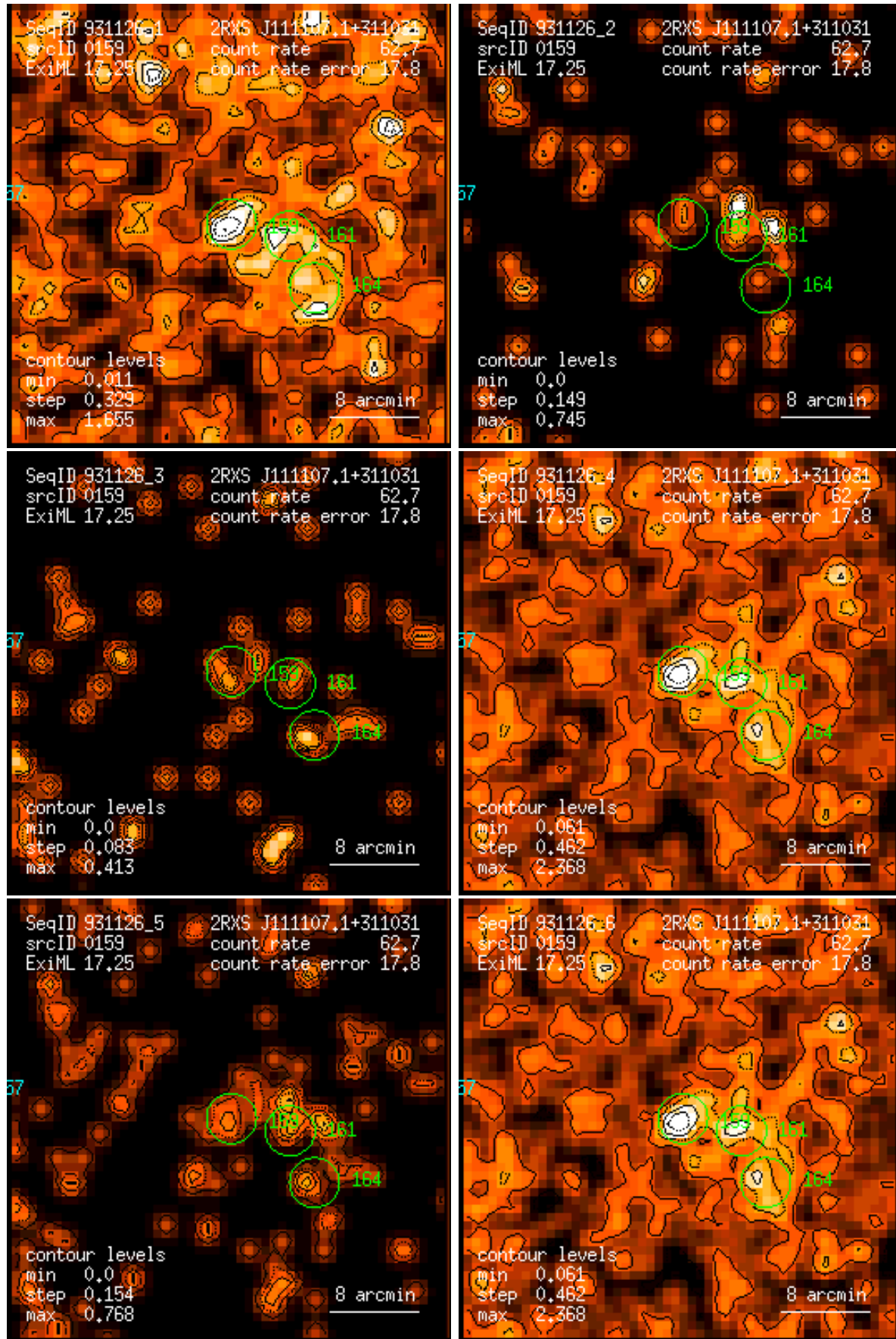
Figure 159: RASS 931126: detection 0159: band rate images, Gaussian filter: (1) PSPC channels 11 – 41, (2) 52 – 90, (3) 91 – 201, (4) 11 – 235, (5) 52 – 201, (6) 11 – 201. Broad band rates in counts/ks. Band rate contour levels in counts/ks/arcmin 2 .
