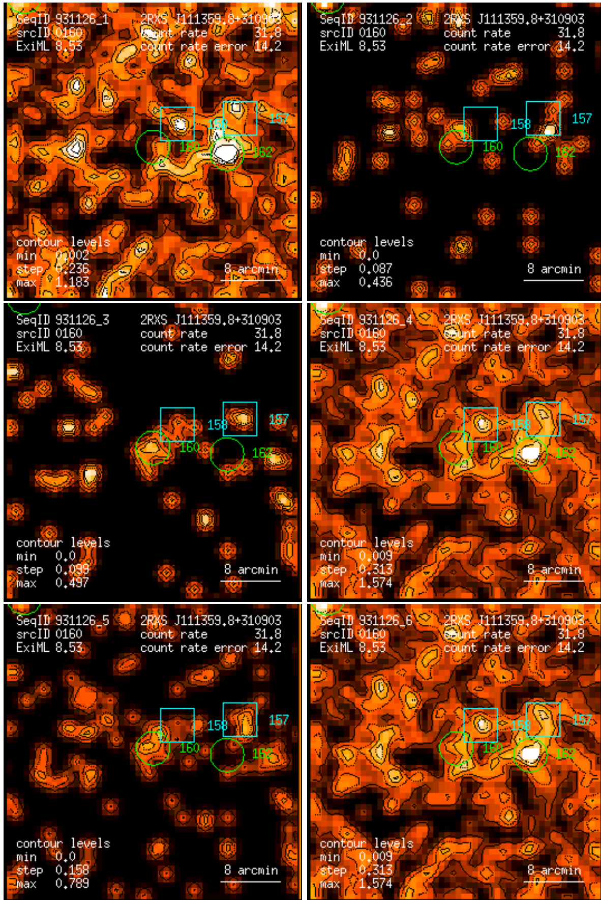
Figure 160: RASS 931126: detection 0160: band rate images, Gaussian filter: (1) PSPC channels 11 – 41, (2) 52 – 90, (3) 91 – 201, (4) 11 – 235, (5) 52 – 201, (6) 11 – 201. Broad band rates in counts/ks. Band rate contour levels in counts/ks/arcmin 2 .
