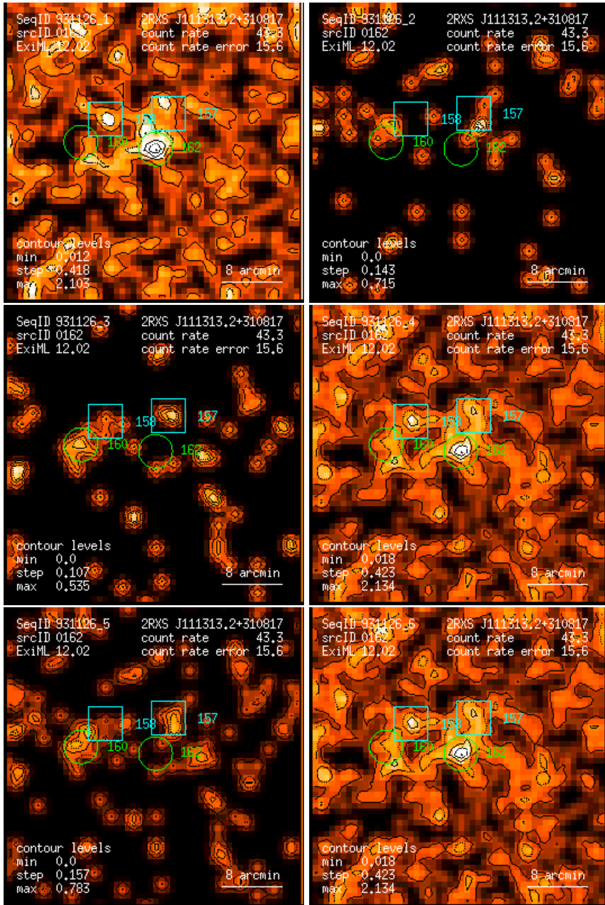
Figure 162: RASS 931126: detection 0162: band rate images, Gaussian filter: (1) PSPC channels 11 – 41, (2) 52 – 90, (3) 91 – 201, (4) 11 – 235, (5) 52 – 201, (6) 11 – 201. Broad band rates in counts/ks. Band rate contour levels in counts/ks/arcmin 2 .
