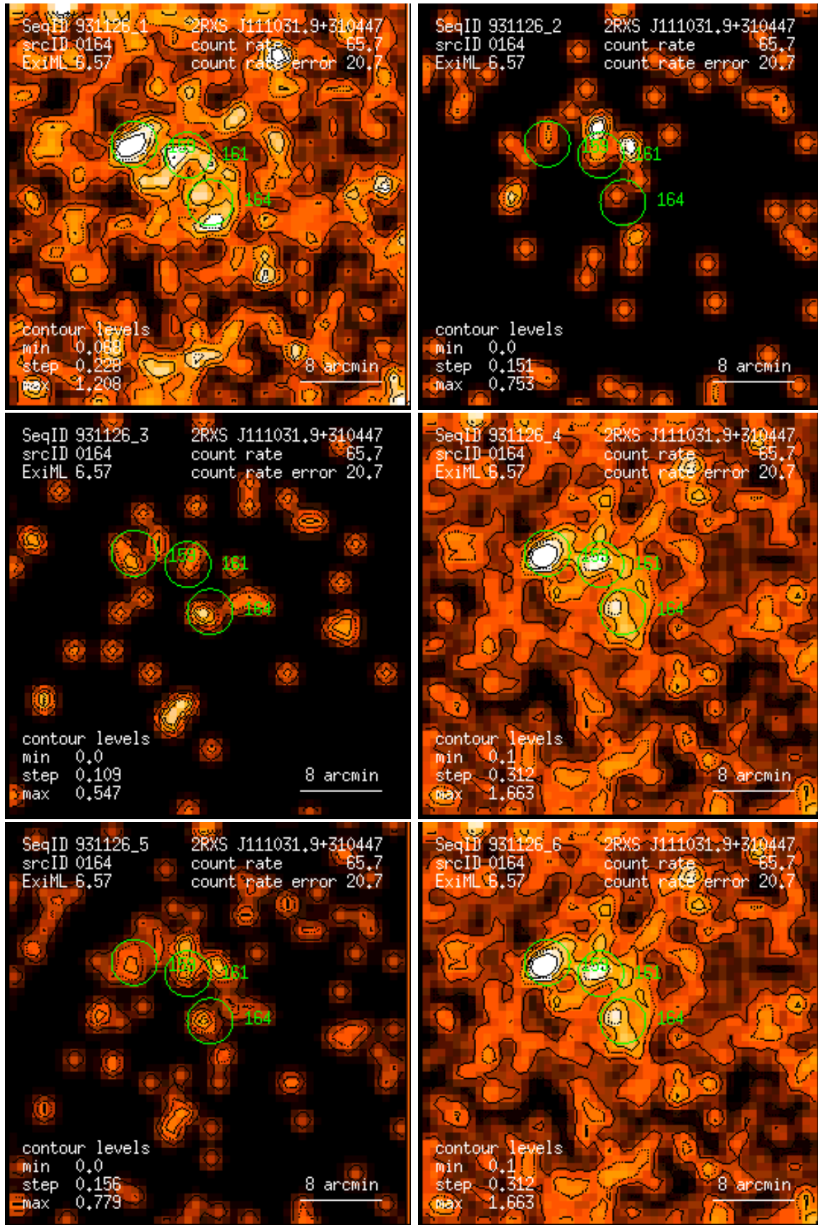
Figure 164: RASS 931126: detection 0164: band rate images, Gaussian filter: (1) PSPC channels 11 – 41, (2) 52 – 90, (3) 91 – 201, (4) 11 – 235, (5) 52 – 201, (6) 11 – 201. Broad band rates in counts/ks. Band rate contour levels in counts/ks/arcmin 2 .
