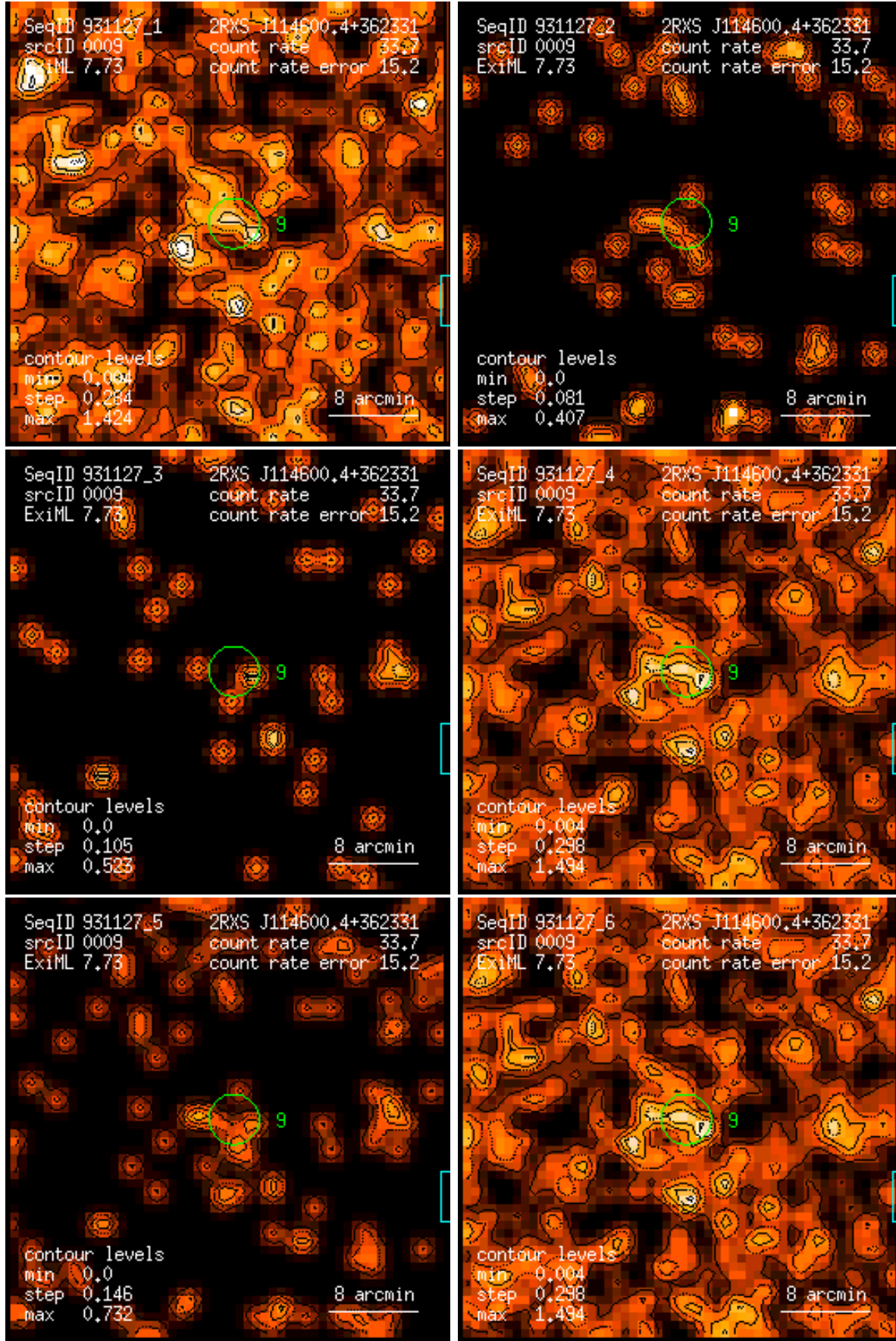
Figure 9: RASS 931127: detection 0009: band rate images, Gaussian filter: (1) PSPC channels 11 – 41, (2) 52 – 90, (3) 91 – 201, (4) 11 – 235, (5) 52 – 201, (6) 11 – 201. Broad band rates in counts/ks. Band rate contour levels in counts/ks/arcmin 2 .
