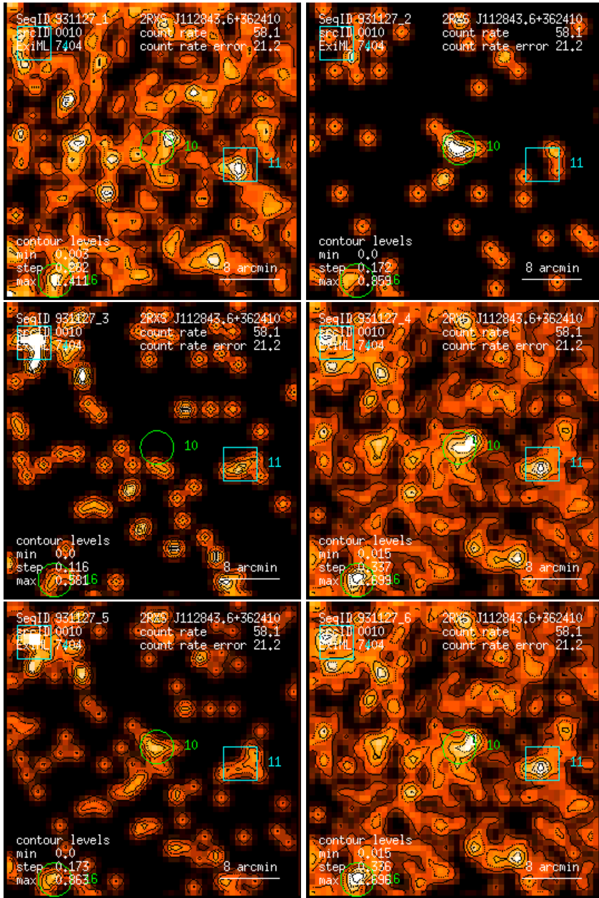
Figure 10: RASS 931127: detection 0010: band rate images, Gaussian filter: (1) PSPC channels 11 – 41, (2) 52 – 90, (3) 91 – 201, (4) 11 – 235, (5) 52 – 201, (6) 11 – 201. Broad band rates in counts/ks. Band rate contour levels in counts/ks/arcmin 2 .
