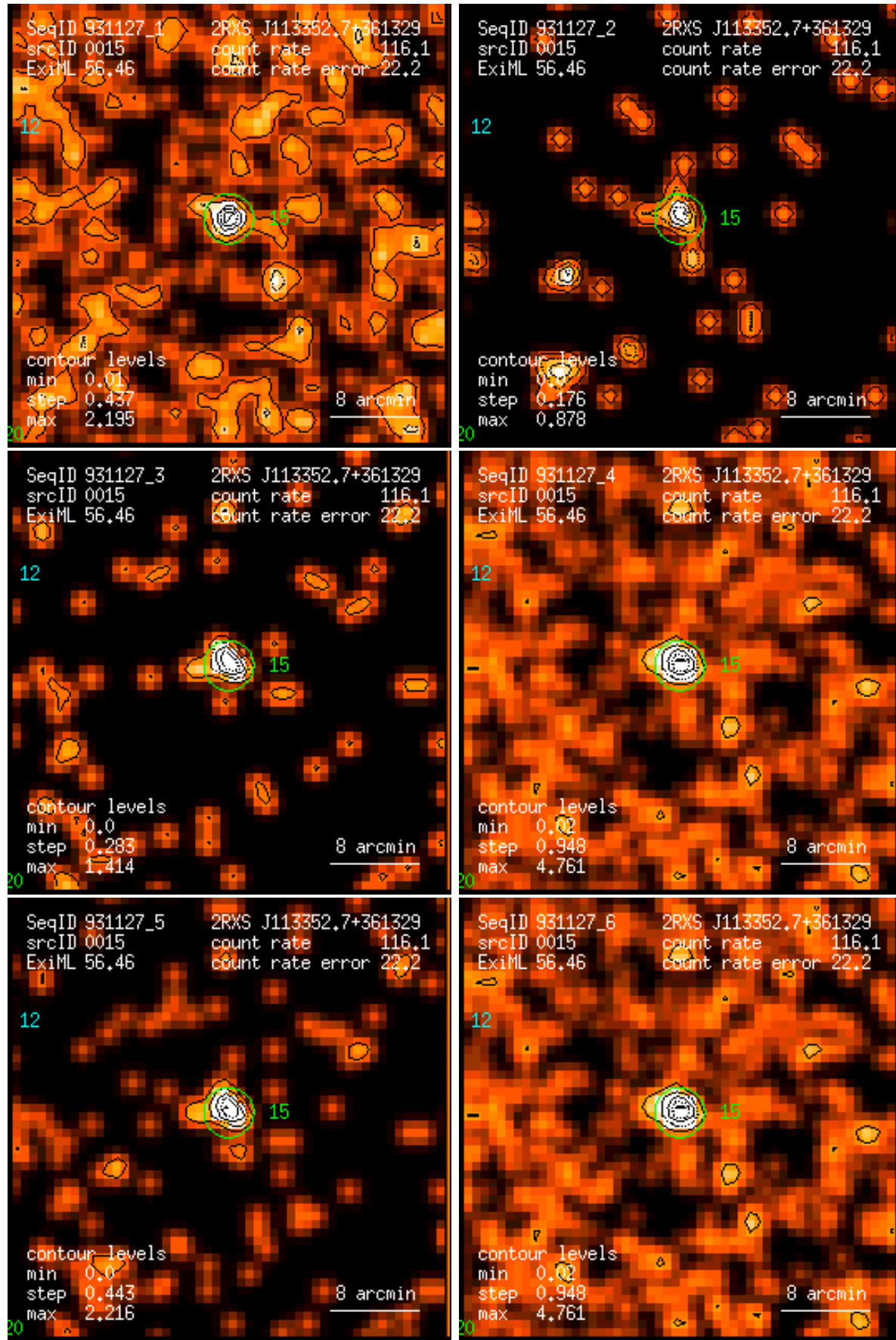
Figure 15: RASS 931127: detection 0015: band rate images, Gaussian filter: (1) PSPC channels 11 – 41, (2) 52 – 90, (3) 91 – 201, (4) 11 – 235, (5) 52 – 201, (6) 11 – 201. Broad band rates in counts/ks. Band rate contour levels in counts/ks/arcmin 2 .
