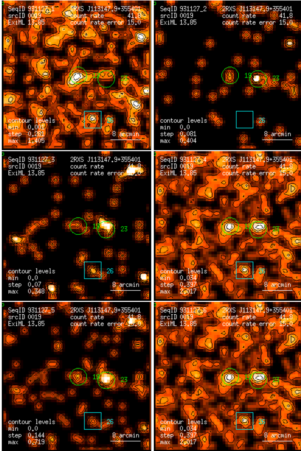
Figure 19: RASS 931127: detection 0019: band rate images, Gaussian filter: (1) PSPC channels 11 – 41, (2) 52 – 90, (3) 91 – 201, (4) 11 – 235, (5) 52 – 201, (6) 11 – 201. Broad band rates in counts/ks. Band rate contour levels in counts/ks/arcmin 2 .
