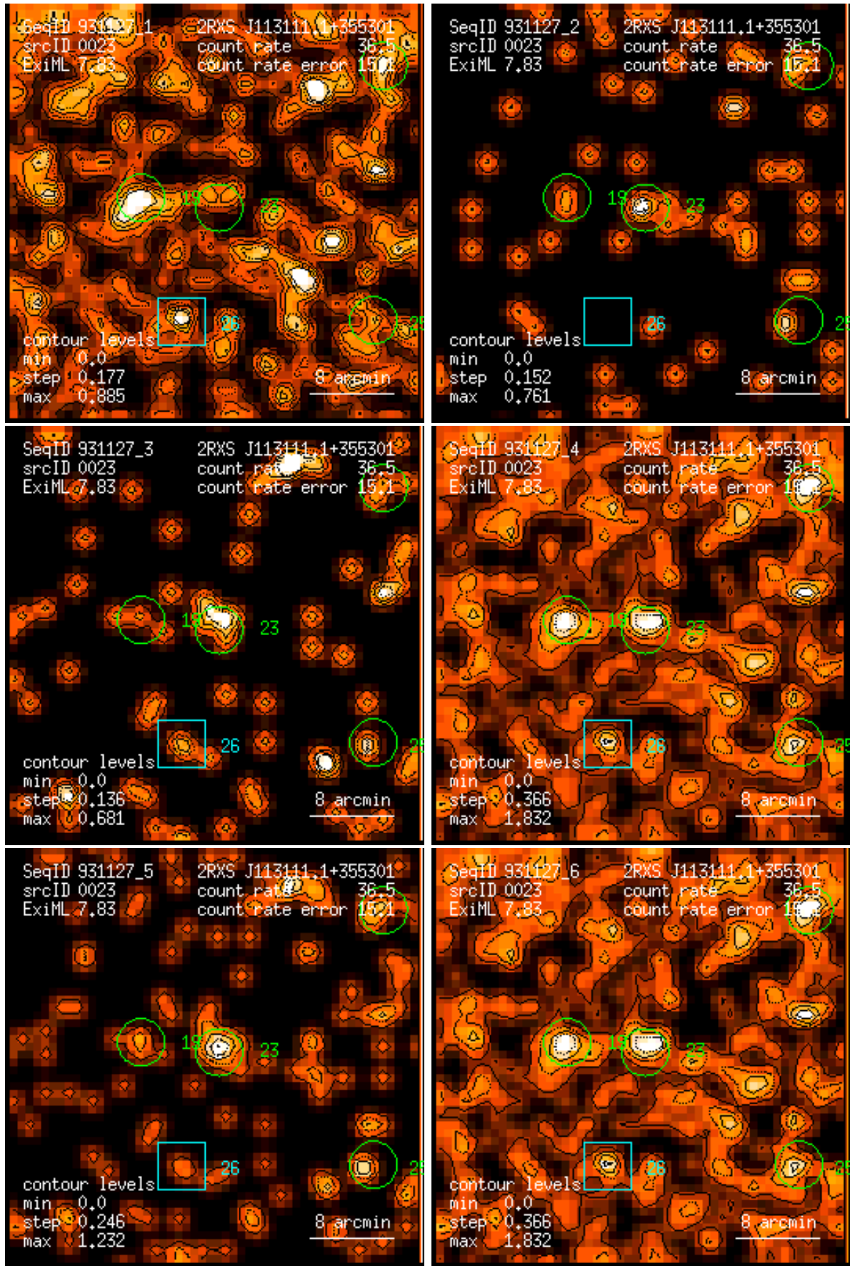
Figure 23: RASS 931127: detection 0023: band rate images, Gaussian filter: (1) PSPC channels 11 – 41, (2) 52 – 90, (3) 91 – 201, (4) 11 – 235, (5) 52 – 201, (6) 11 – 201. Broad band rates in counts/ks. Band rate contour levels in counts/ks/arcmin 2 .
