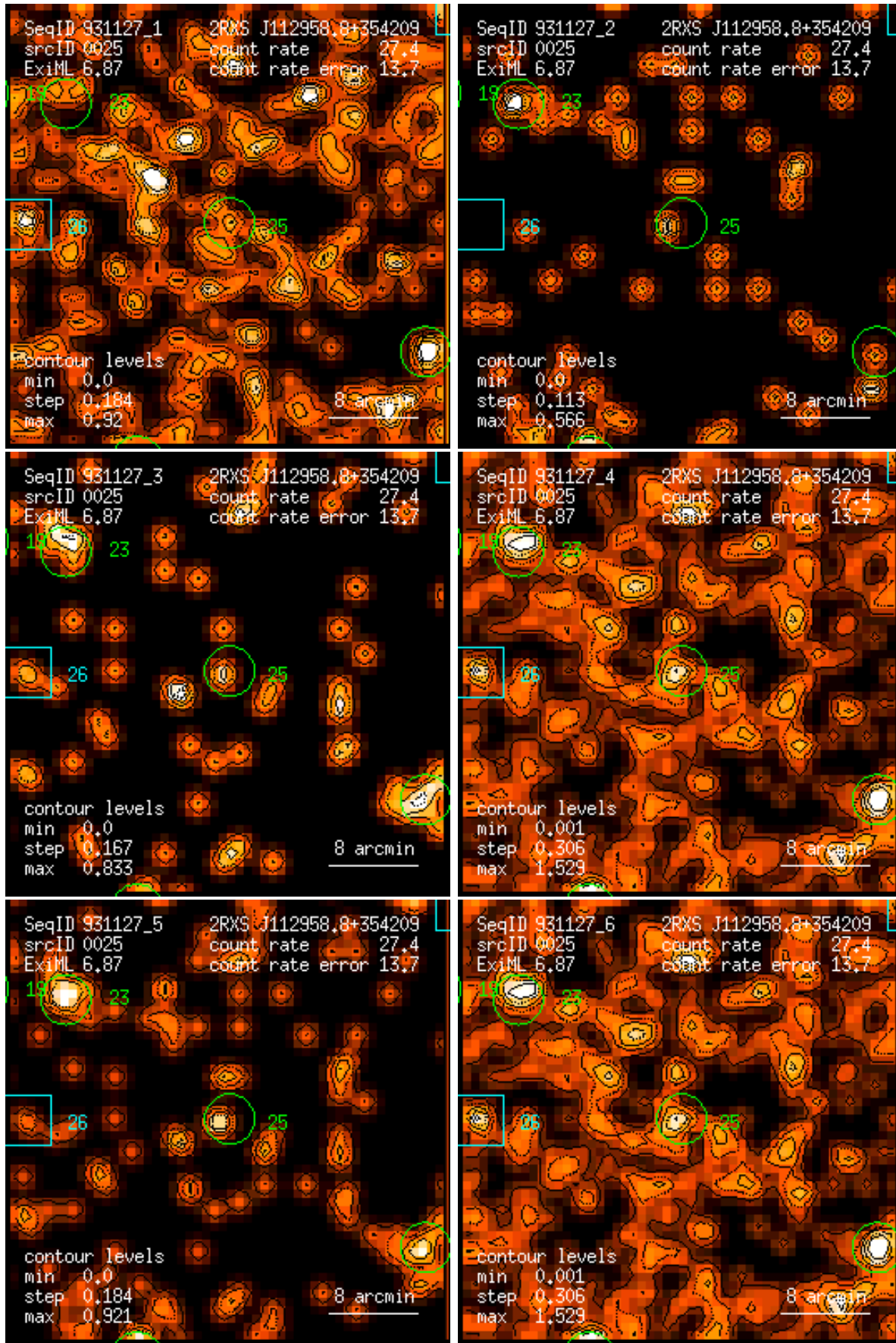
Figure 25: RASS 931127: detection 0025: band rate images, Gaussian filter: (1) PSPC channels 11 – 41, (2) 52 – 90, (3) 91 – 201, (4) 11 – 235, (5) 52 – 201, (6) 11 – 201. Broad band rates in counts/ks. Band rate contour levels in counts/ks/arcmin 2 .
