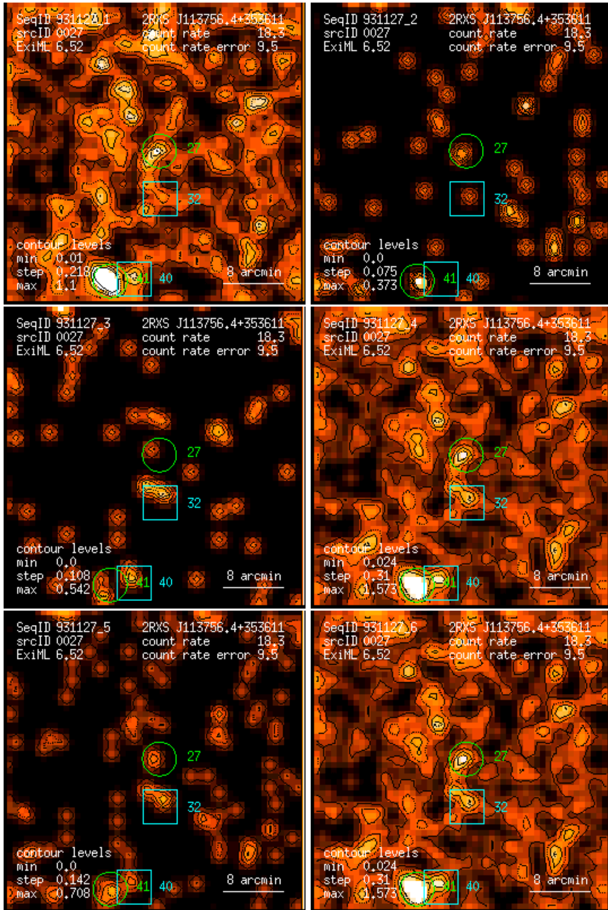
Figure 27: RASS 931127: detection 0027: band rate images, Gaussian filter: (1) PSPC channels 11 – 41, (2) 52 – 90, (3) 91 – 201, (4) 11 – 235, (5) 52 – 201, (6) 11 – 201. Broad band rates in counts/ks. Band rate contour levels in counts/ks/arcmin 2 .
