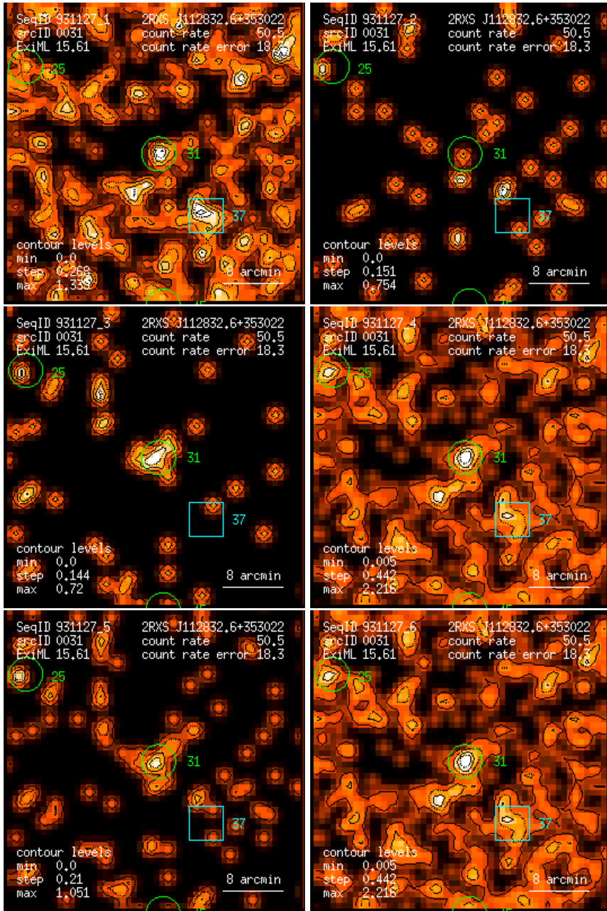
Figure 31: RASS 931127: detection 0031: band rate images, Gaussian filter: (1) PSPC channels 11 – 41, (2) 52 – 90, (3) 91 – 201, (4) 11 – 235, (5) 52 – 201, (6) 11 – 201. Broad band rates in counts/ks. Band rate contour levels in counts/ks/arcmin 2 .
