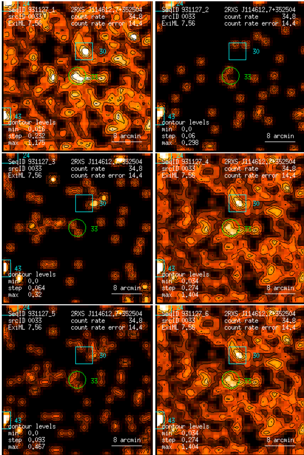
Figure 33: RASS 931127: detection 0033: band rate images, Gaussian filter: (1) PSPC channels 11 – 41, (2) 52 – 90, (3) 91 – 201, (4) 11 – 235, (5) 52 – 201, (6) 11 – 201. Broad band rates in counts/ks. Band rate contour levels in counts/ks/arcmin 2 .
