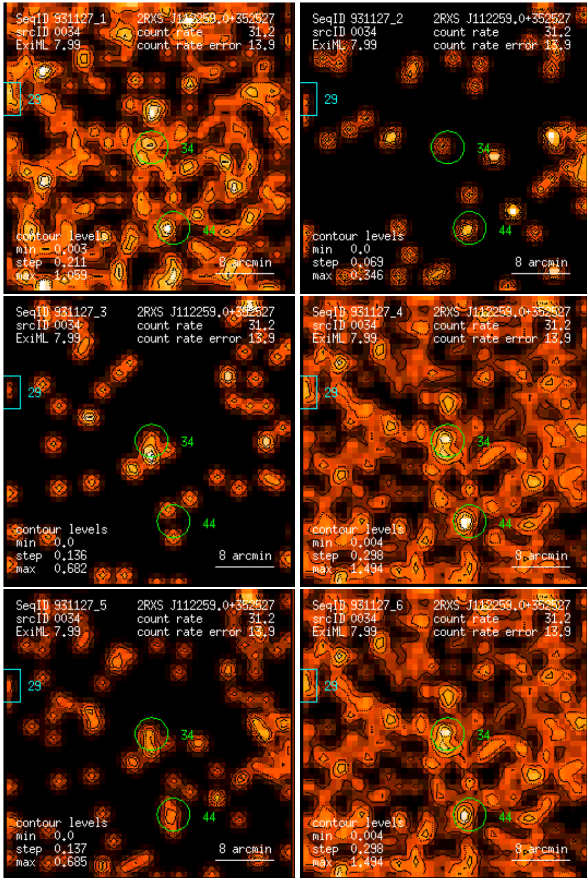
Figure 34: RASS 931127: detection 0034: band rate images, Gaussian filter: (1) PSPC channels 11 – 41, (2) 52 – 90, (3) 91 – 201, (4) 11 – 235, (5) 52 – 201, (6) 11 – 201. Broad band rates in counts/ks. Band rate contour levels in counts/ks/arcmin 2 .
