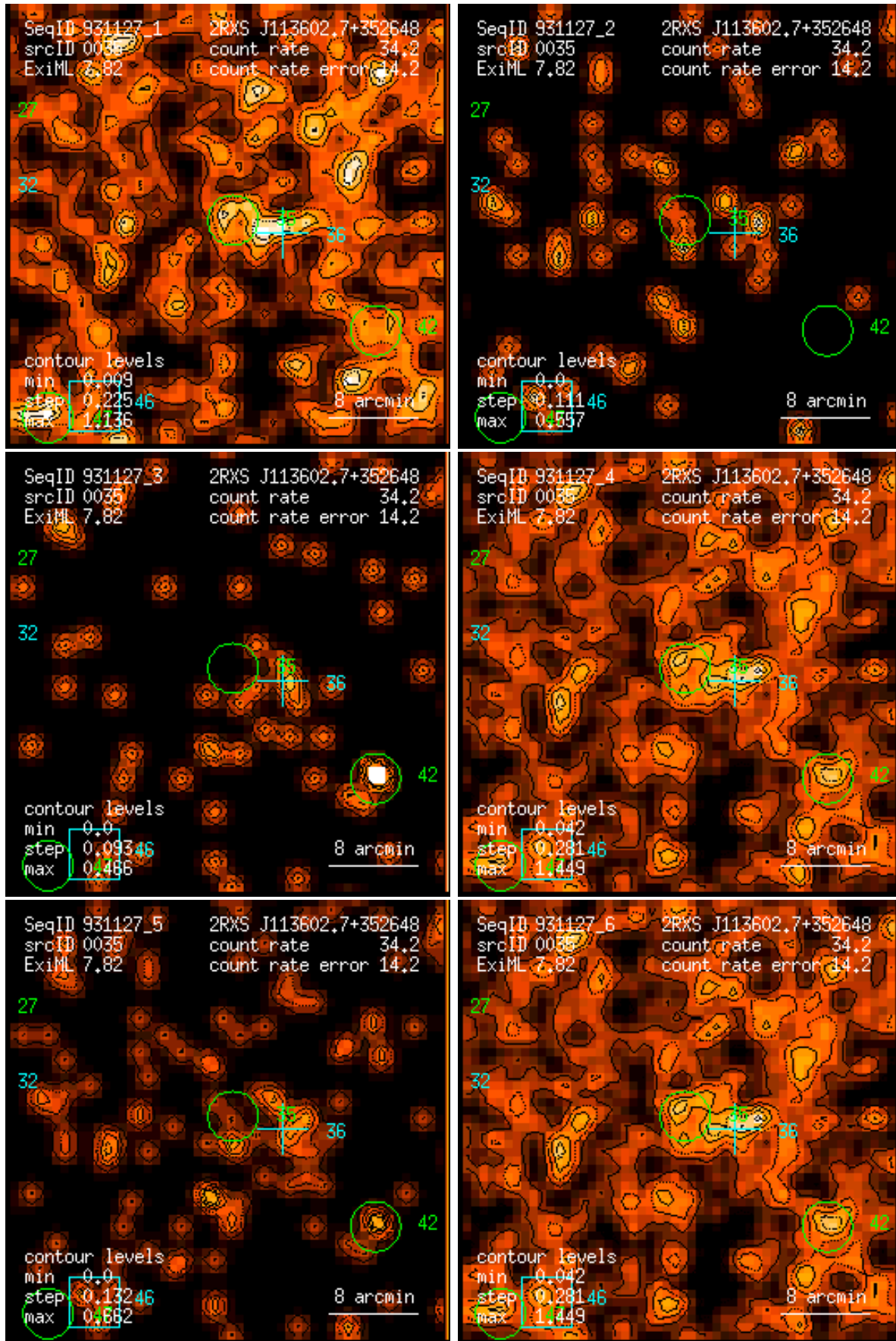
Figure 35: RASS 931127: detection 0035: band rate images, Gaussian filter: (1) PSPC channels 11 – 41, (2) 52 – 90, (3) 91 – 201, (4) 11 – 235, (5) 52 – 201, (6) 11 – 201. Broad band rates in counts/ks. Band rate contour levels in counts/ks/arcmin 2 .
