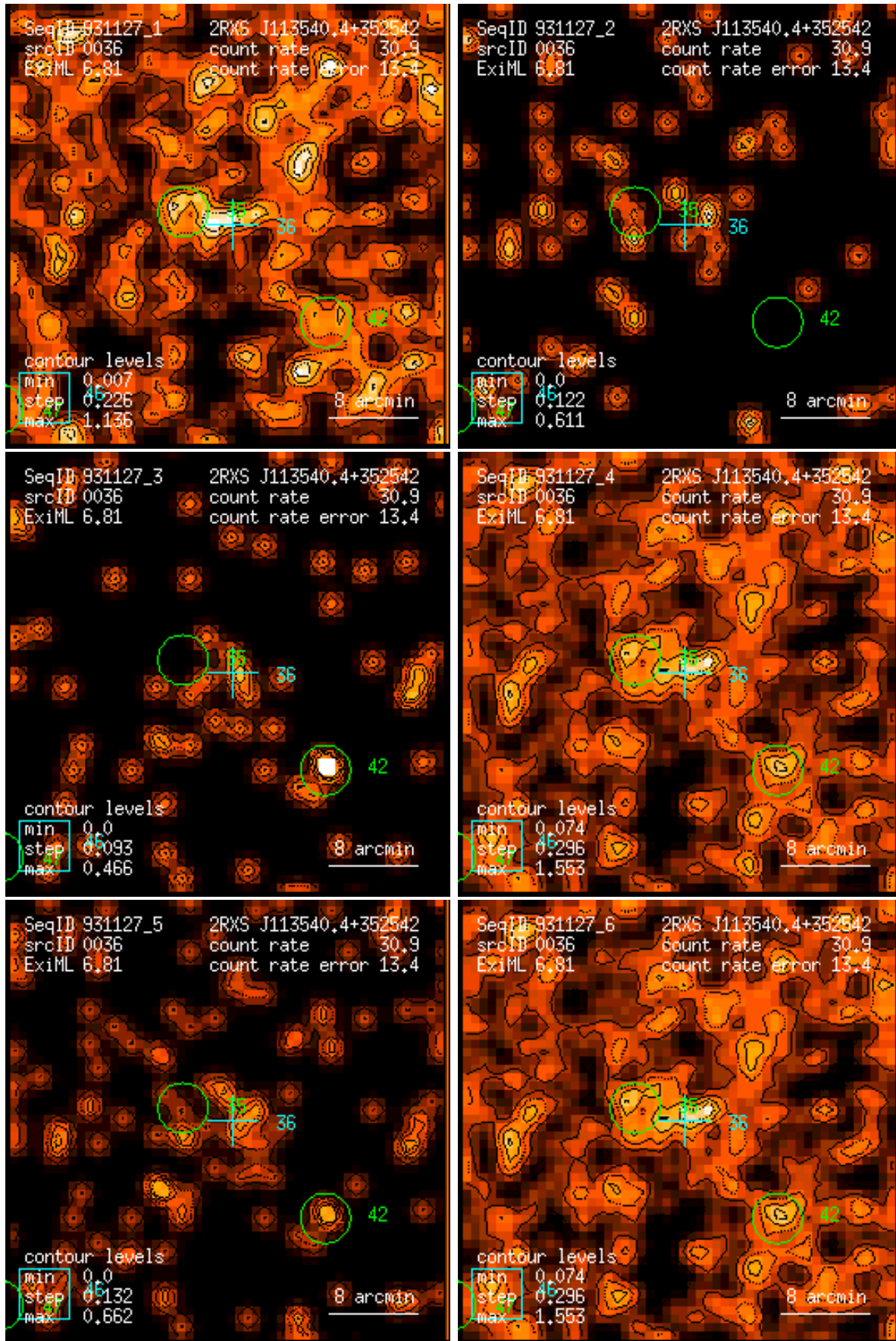
Figure 36: RASS 931127: detection 0036: band rate images, Gaussian filter: (1) PSPC channels 11 – 41, (2) 52 – 90, (3) 91 – 201, (4) 11 – 235, (5) 52 – 201, (6) 11 – 201. Broad band rates in counts/ks. Band rate contour levels in counts/ks/arcmin 2 .
