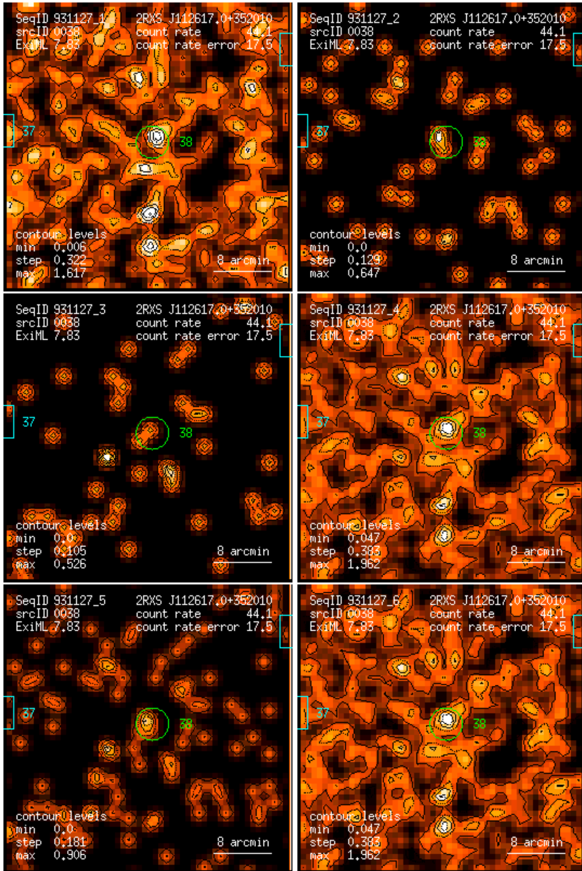
Figure 38: RASS 931127: detection 0038: band rate images, Gaussian filter: (1) PSPC channels 11 – 41, (2) 52 – 90, (3) 91 – 201, (4) 11 – 235, (5) 52 – 201, (6) 11 – 201. Broad band rates in counts/ks. Band rate contour levels in counts/ks/arcmin 2 .
