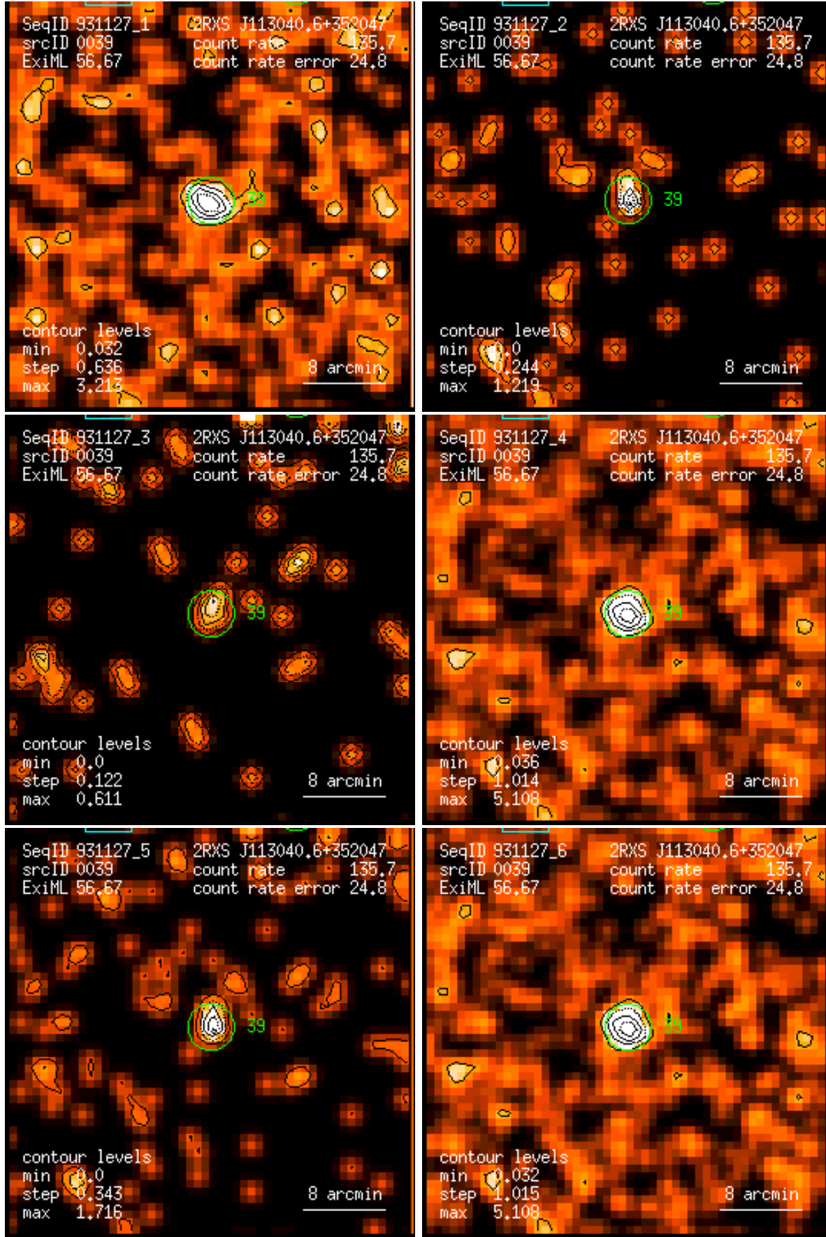
Figure 39: RASS 931127: detection 0039: band rate images, Gaussian filter: (1) PSPC channels 11 – 41, (2) 52 – 90, (3) 91 – 201, (4) 11 – 235, (5) 52 – 201, (6) 11 – 201. Broad band rates in counts/ks. Band rate contour levels in counts/ks/arcmin 2 .
