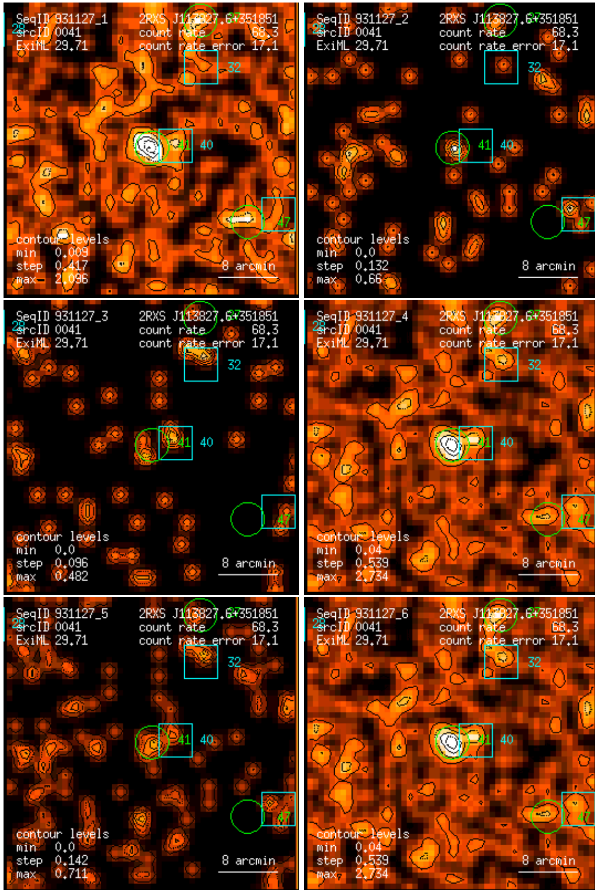
Figure 41: RASS 931127: detection 0041: band rate images, Gaussian filter: (1) PSPC channels 11 – 41, (2) 52 – 90, (3) 91 – 201, (4) 11 – 235, (5) 52 – 201, (6) 11 – 201. Broad band rates in counts/ks. Band rate contour levels in counts/ks/arcmin 2 .
