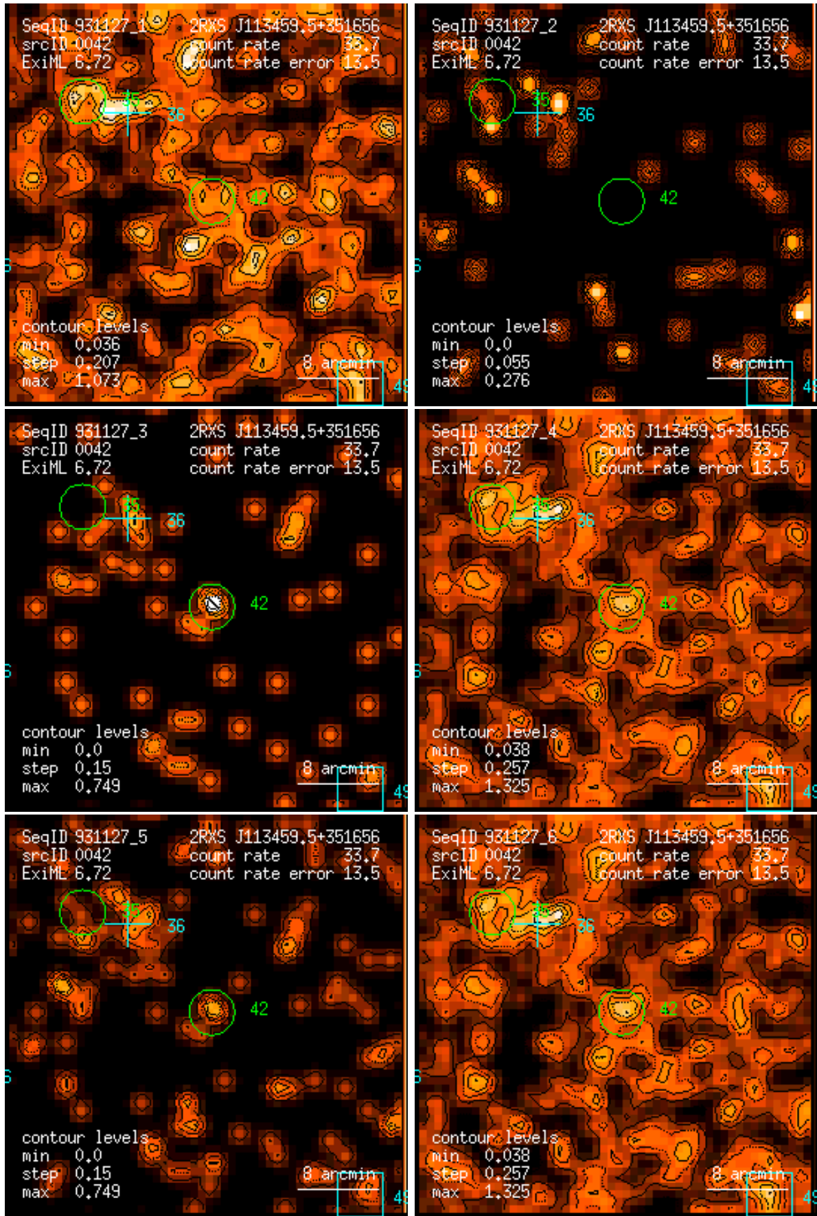
Figure 42: RASS 931127: detection 0042: band rate images, Gaussian filter: (1) PSPC channels 11 – 41, (2) 52 – 90, (3) 91 – 201, (4) 11 – 235, (5) 52 – 201, (6) 11 – 201. Broad band rates in counts/ks. Band rate contour levels in counts/ks/arcmin 2 .
