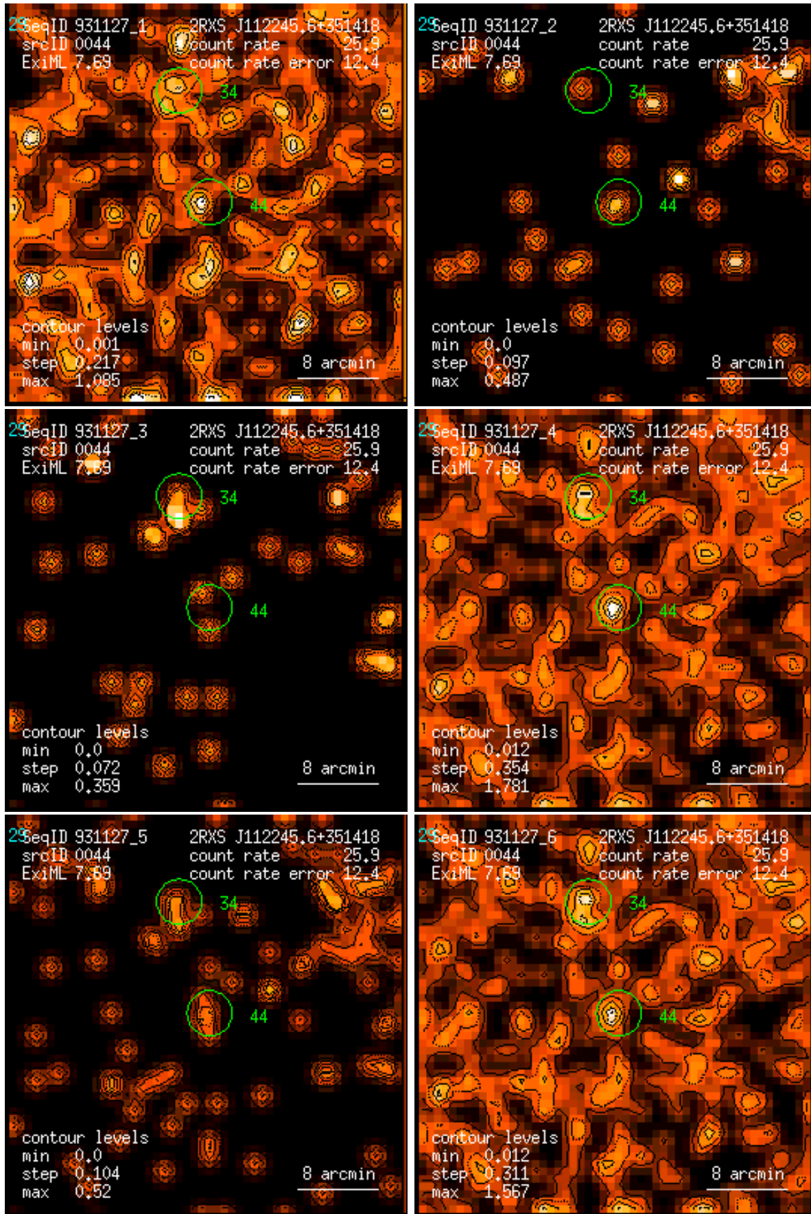
Figure 44: RASS 931127: detection 0044: band rate images, Gaussian filter: (1) PSPC channels 11 – 41, (2) 52 – 90, (3) 91 – 201, (4) 11 – 235, (5) 52 – 201, (6) 11 – 201. Broad band rates in counts/ks. Band rate contour levels in counts/ks/arcmin 2 .
