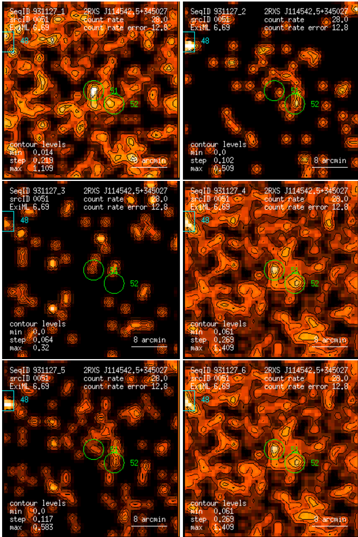
Figure 51: RASS 931127: detection 0051: band rate images, Gaussian filter: (1) PSPC channels 11 – 41, (2) 52 – 90, (3) 91 – 201, (4) 11 – 235, (5) 52 – 201, (6) 11 – 201. Broad band rates in counts/ks. Band rate contour levels in counts/ks/arcmin 2 .
