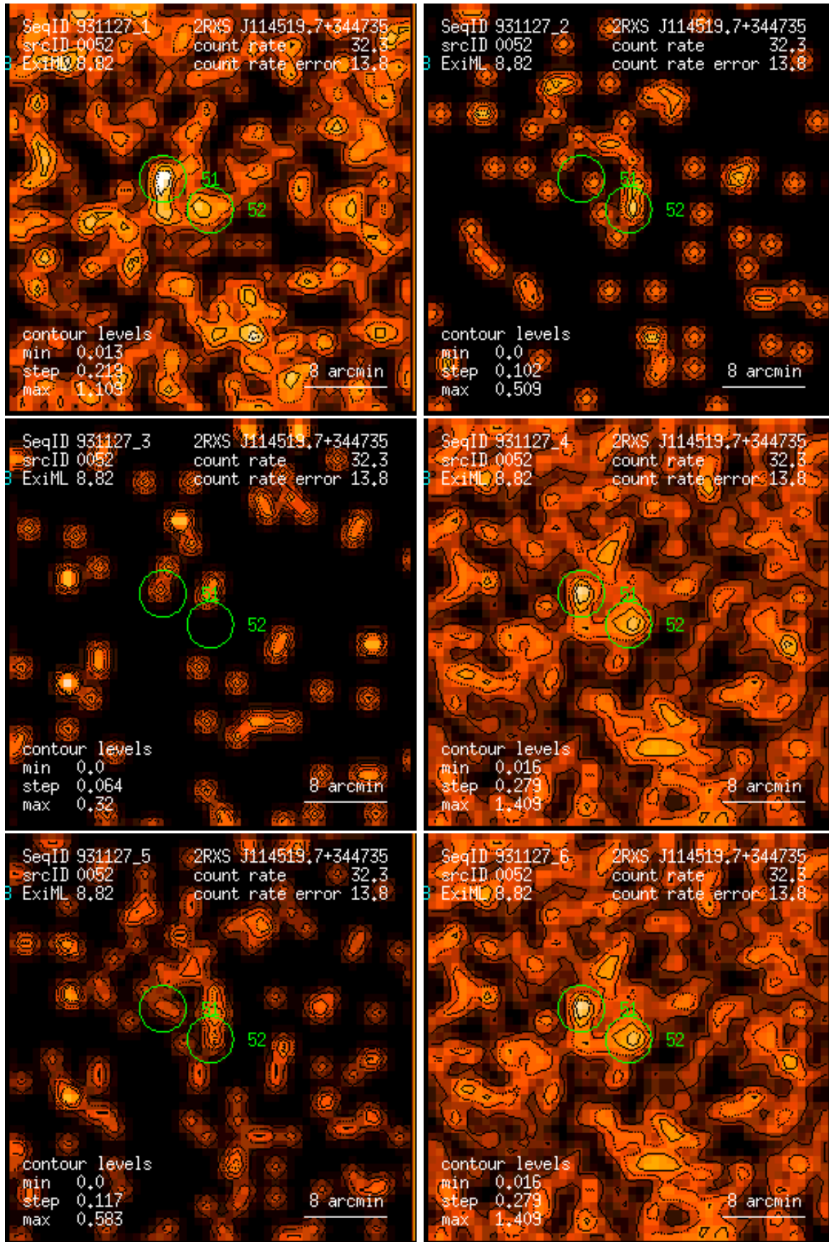
Figure 52: RASS 931127: detection 0052: band rate images, Gaussian filter: (1) PSPC channels 11 – 41, (2) 52 – 90, (3) 91 – 201, (4) 11 – 235, (5) 52 – 201, (6) 11 – 201. Broad band rates in counts/ks. Band rate contour levels in counts/ks/arcmin 2 .
