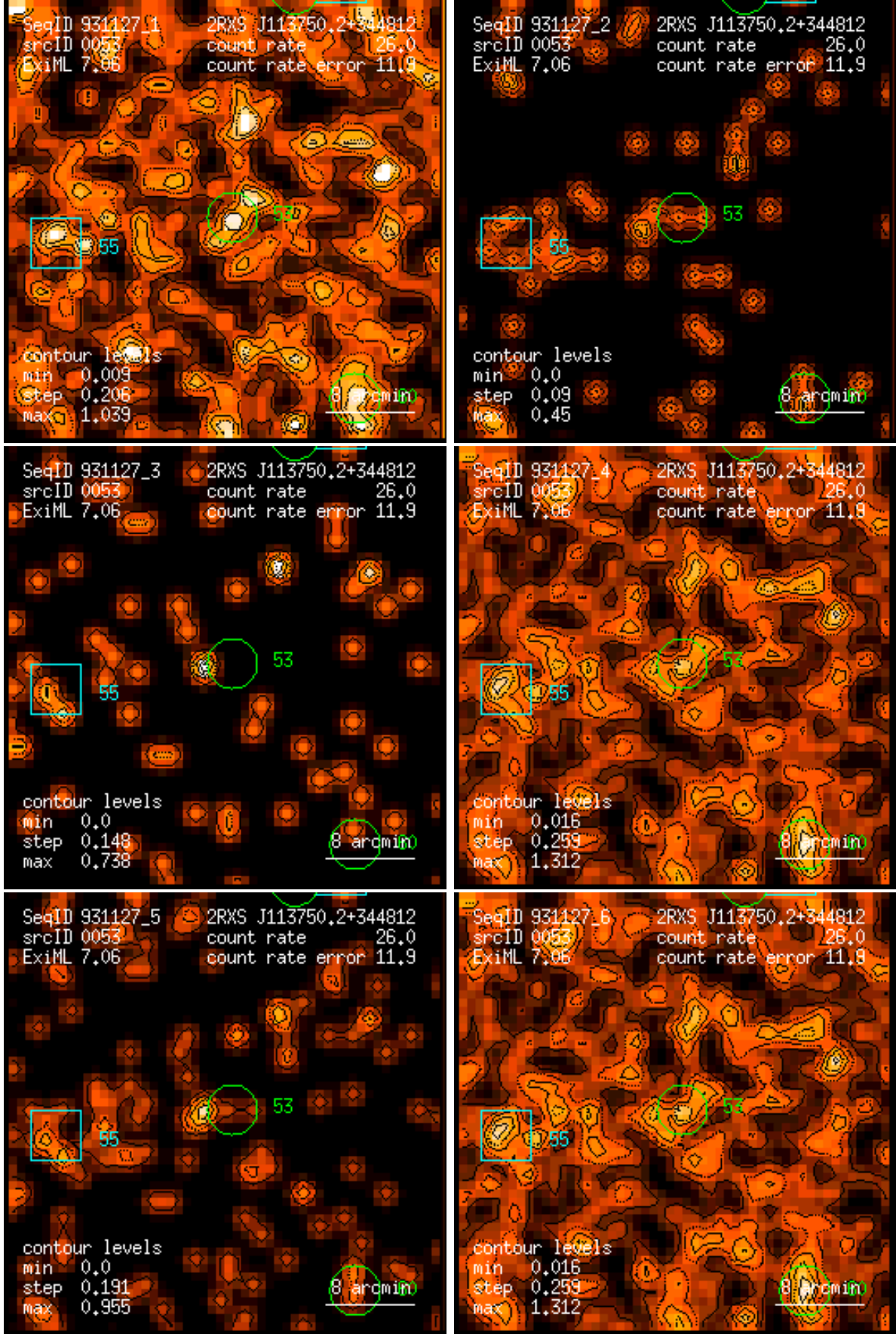
Figure 53: RASS 931127: detection 0053: band rate images, Gaussian filter: (1) PSPC channels 11 – 41, (2) 52 – 90, (3) 91 – 201, (4) 11 – 235, (5) 52 – 201, (6) 11 – 201. Broad band rates in counts/ks. Band rate contour levels in counts/ks/arcmin 2 .
