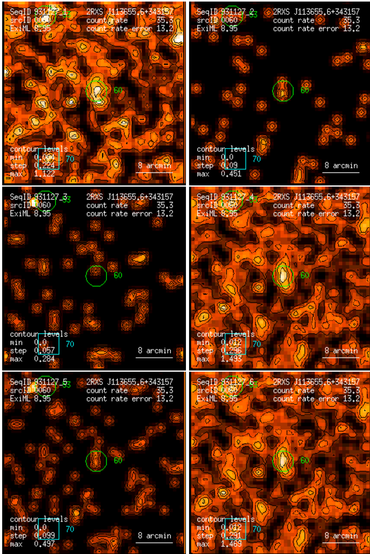
Figure 60: RASS 931127: detection 0060: band rate images, Gaussian filter: (1) PSPC channels 11 – 41, (2) 52 – 90, (3) 91 – 201, (4) 11 – 235, (5) 52 – 201, (6) 11 – 201. Broad band rates in counts/ks. Band rate contour levels in counts/ks/arcmin 2 .
