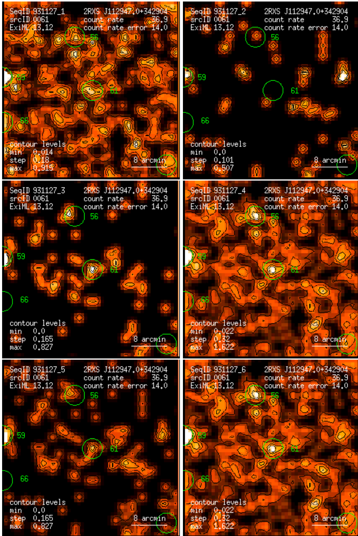
Figure 61: RASS 931127: detection 0061: band rate images, Gaussian filter: (1) PSPC channels 11 – 41, (2) 52 – 90, (3) 91 – 201, (4) 11 – 235, (5) 52 – 201, (6) 11 – 201. Broad band rates in counts/ks. Band rate contour levels in counts/ks/arcmin 2 .
